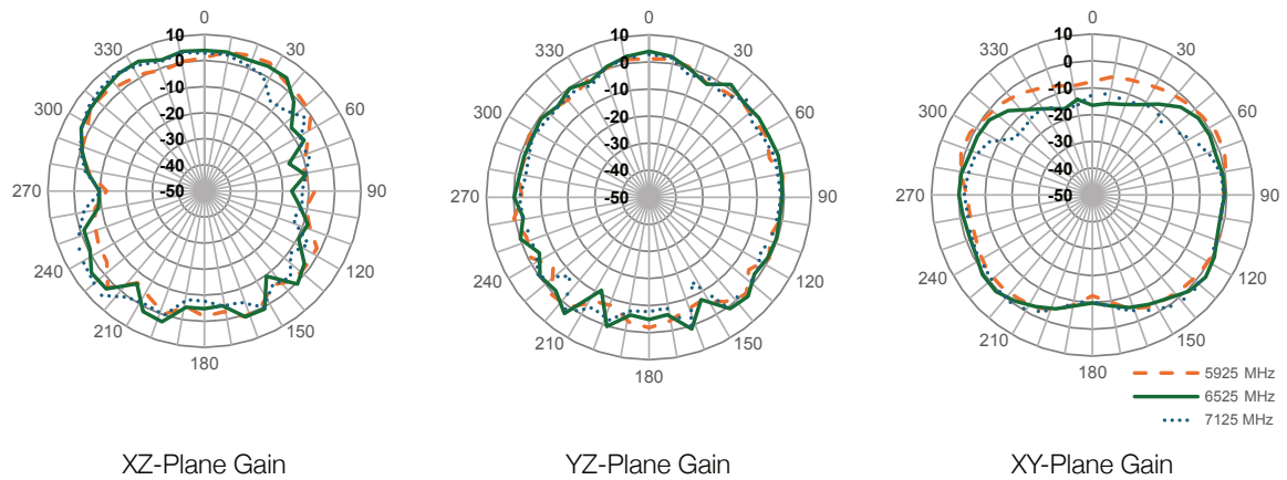
Figure 7. Radiation Patterns for the AC11003 Antenna
