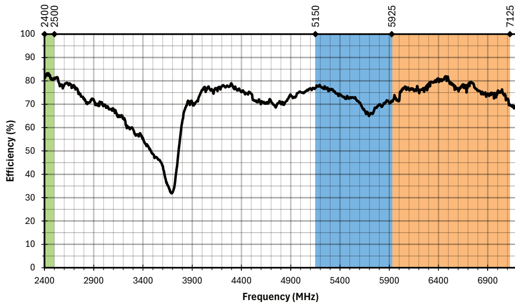
Figure 6. AC11003 Antenna Efficiency
