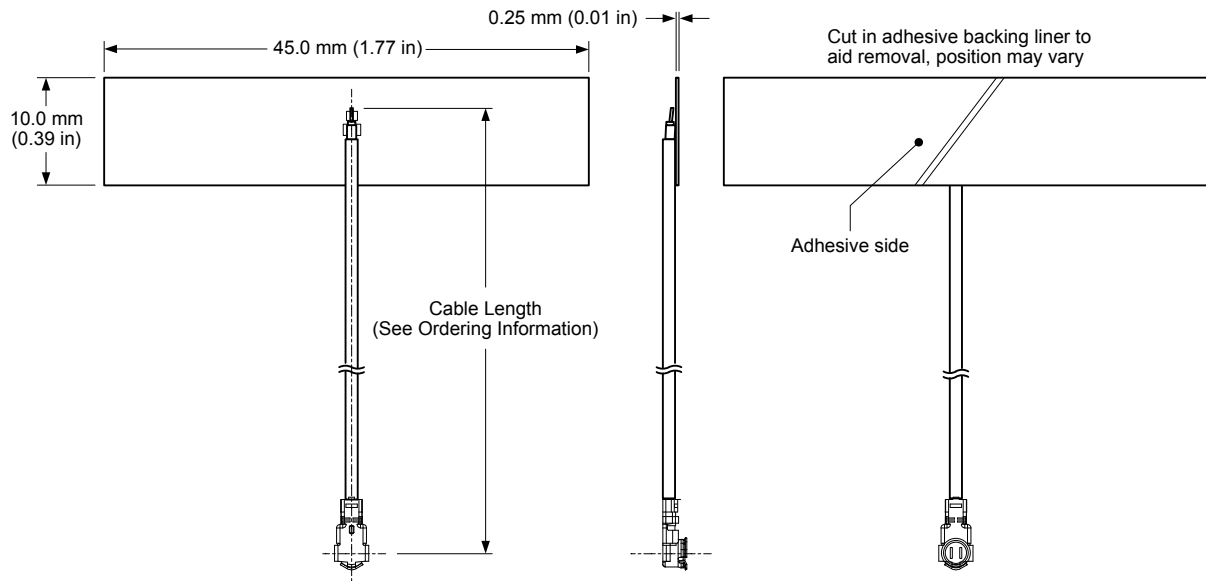
Figure 1. AC11003 Antenna Dimensions
