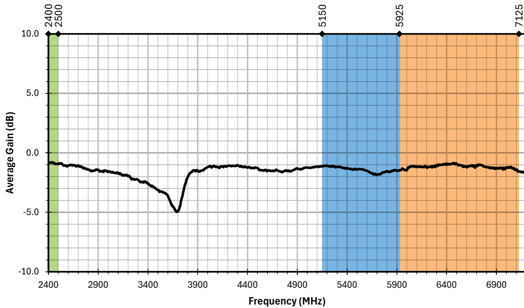
Figure 5. AC11003 Antenna Average Gain
