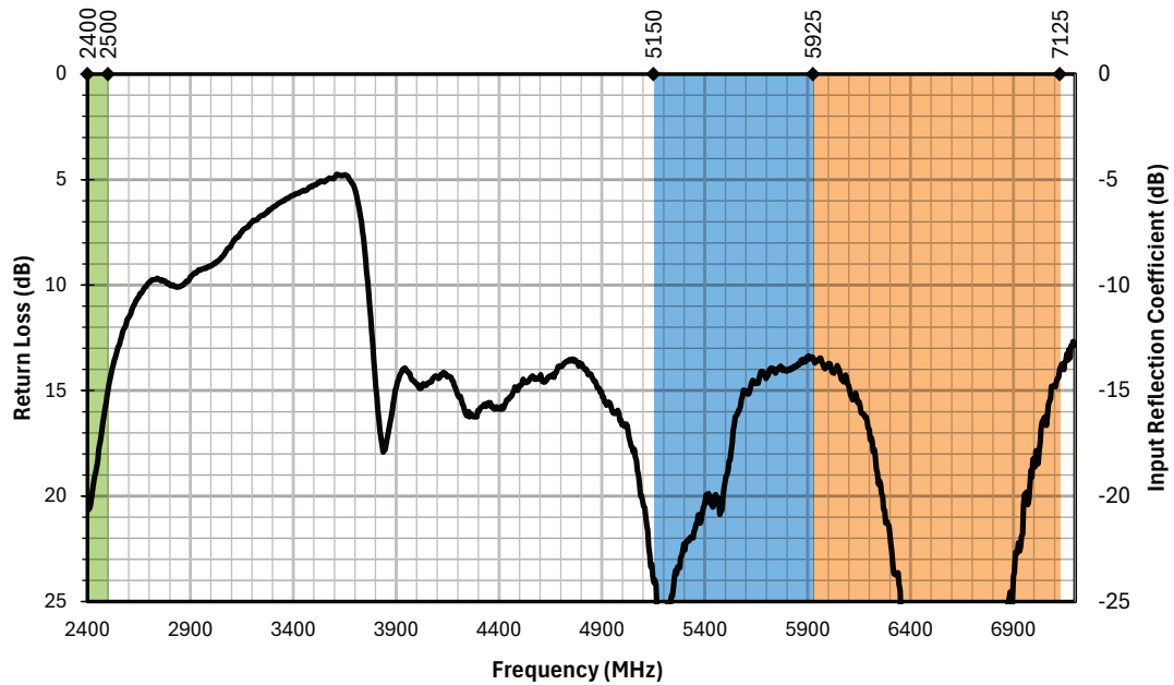
Figure 3. AC11003 Antenna Return Loss
