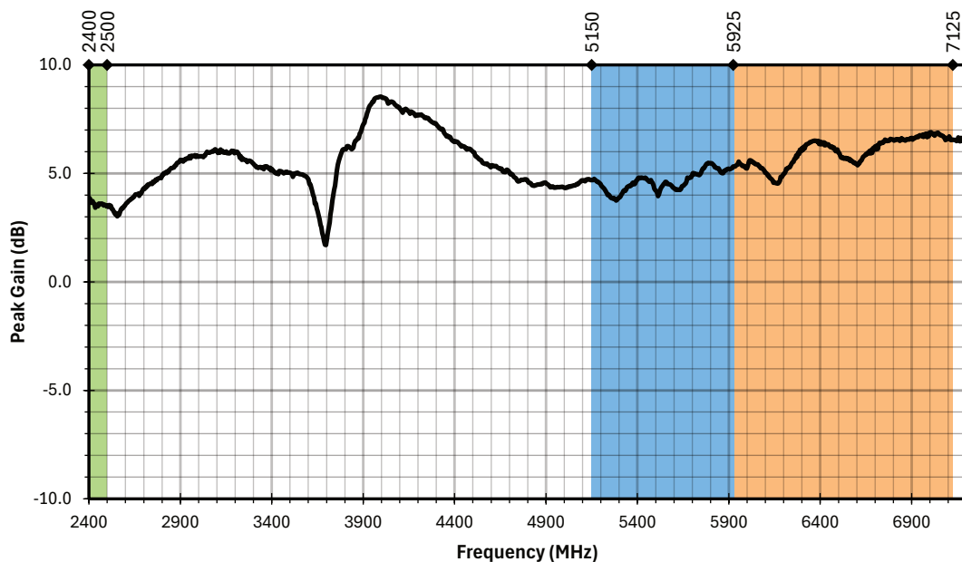
Figure 4. AC11003 Antenna Peak Gain
