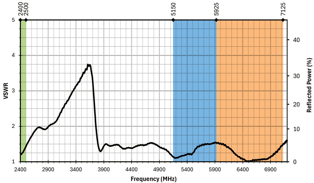
Figure 2. AC11003 Antenna VSWR
