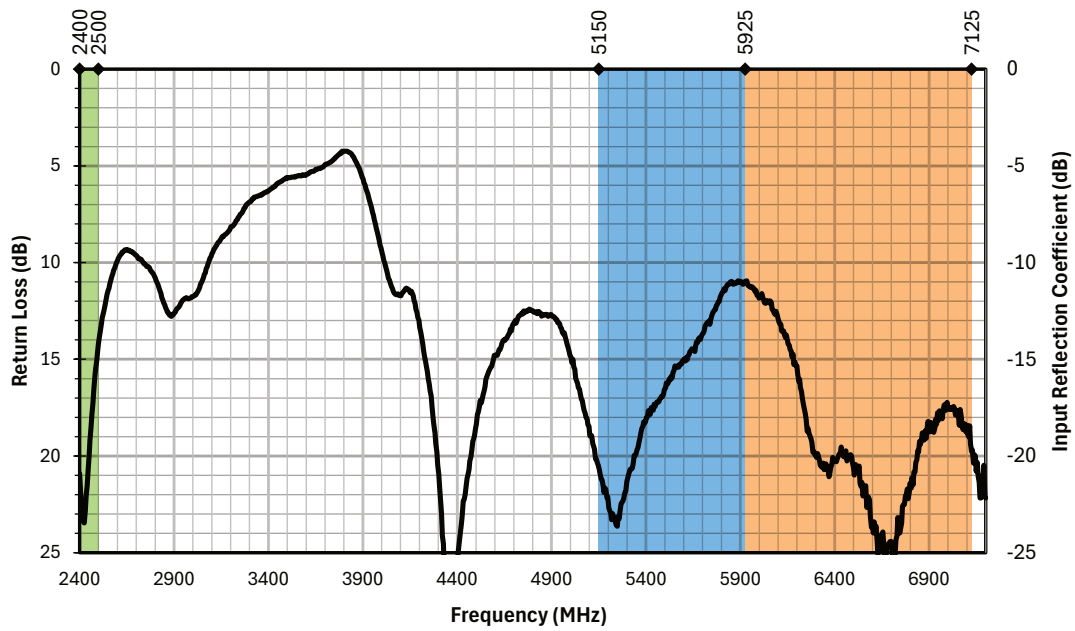
Figure 3. AC11004 Antenna Return Loss
