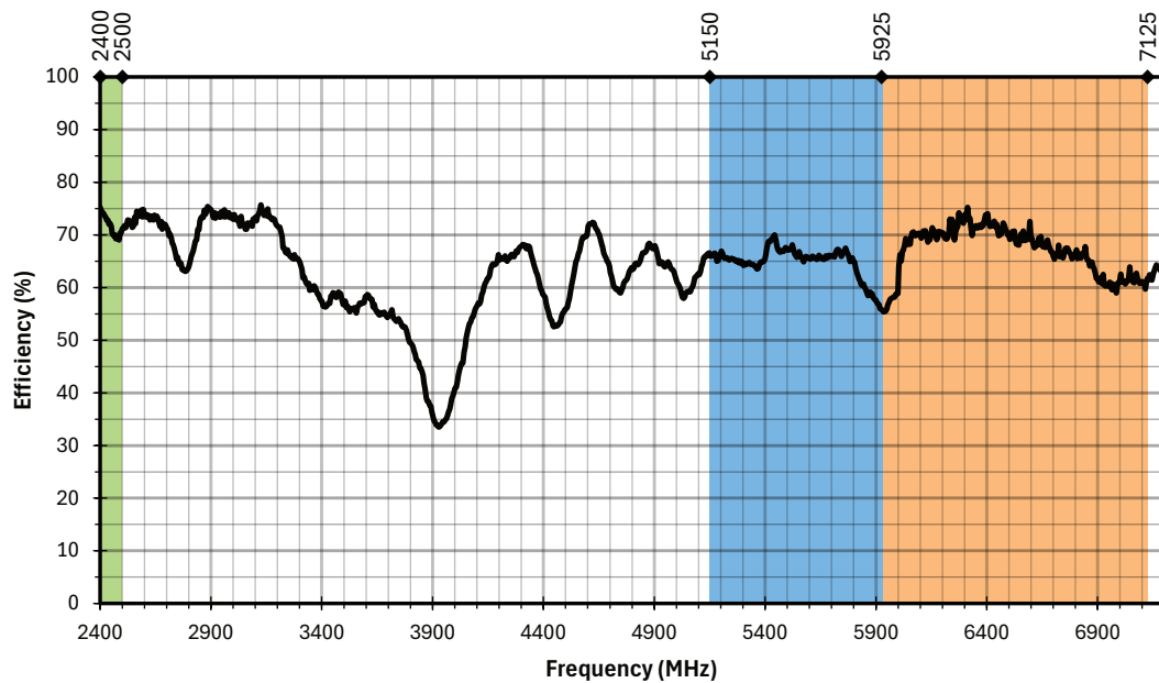
Figure 6. AC11004 Antenna Efficiency
