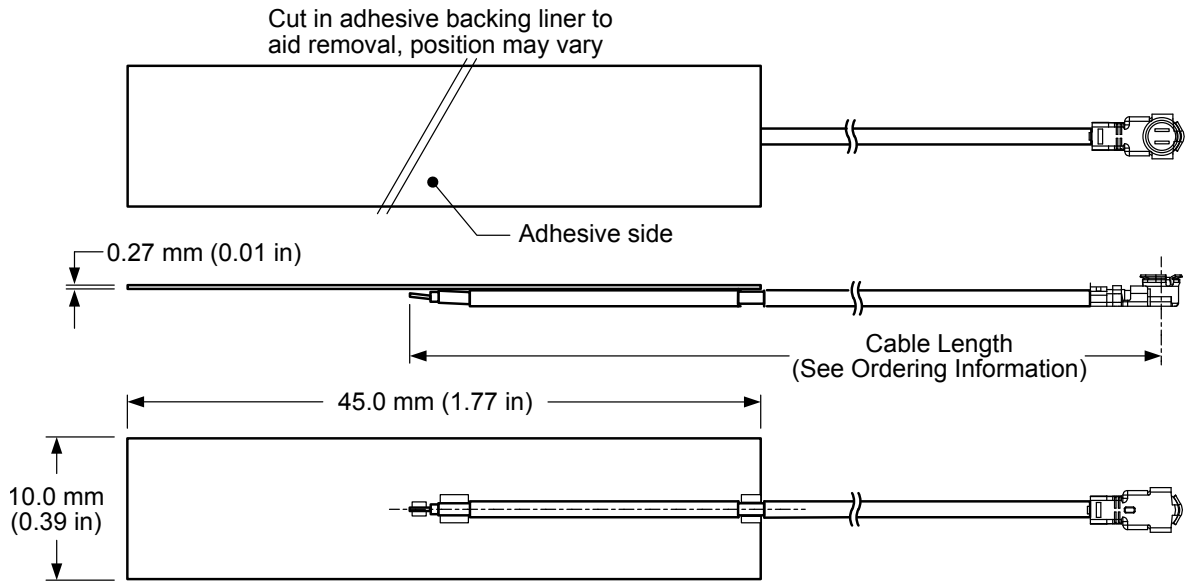
Figure 1. AC11004 Antenna Dimensions
