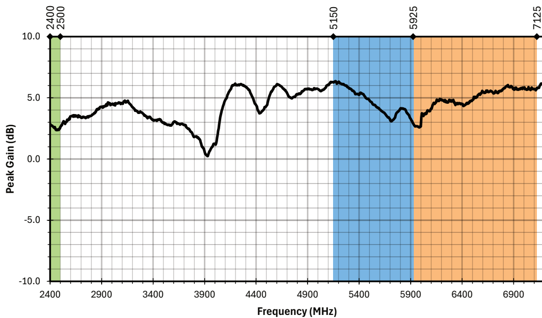
Figure 4. AC11004 Antenna Peak Gain
