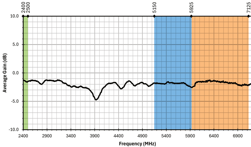
Figure 5. AC11004 Antenna Average Gain
