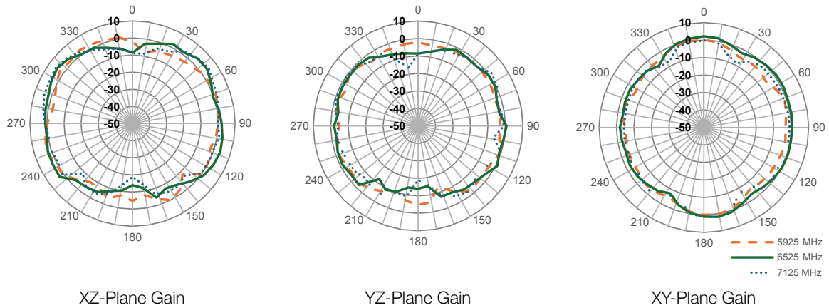
Figure 7. Radiation Patterns for the AC11004 Antenna
