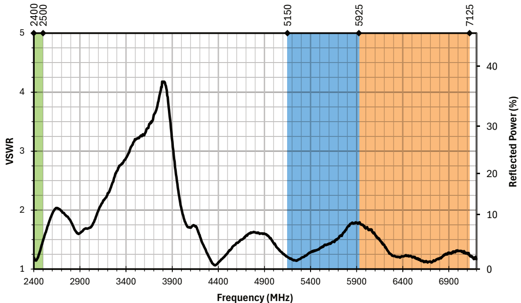
Figure 2. AC11004 Antenna VSWR
