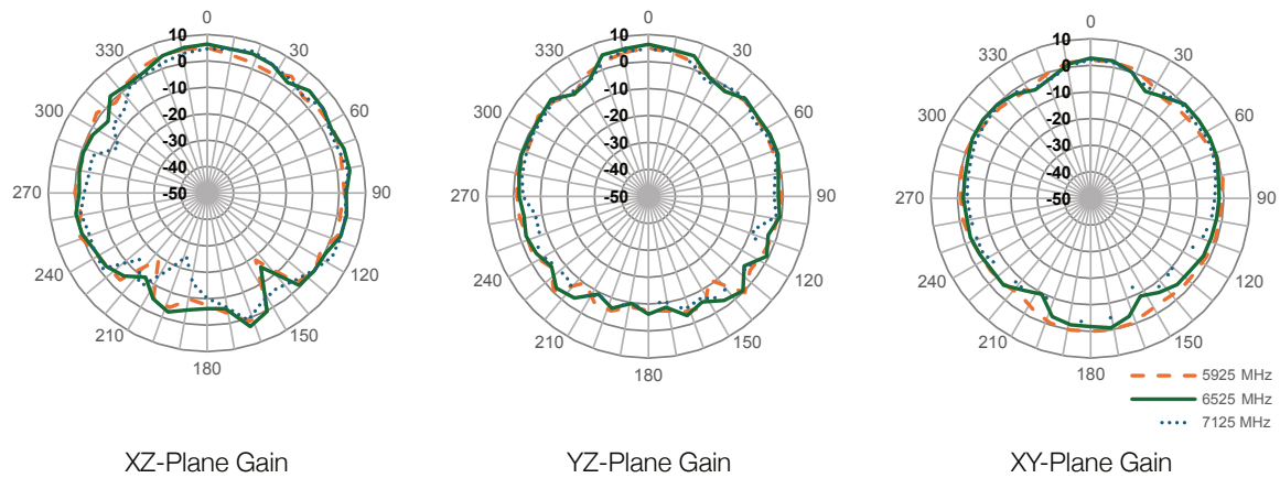
Figure 7. Radiation Patterns for the AC11005 Antenna
