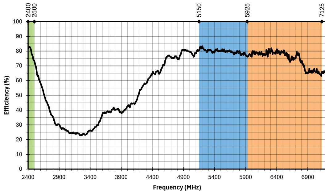
Figure 6. AC11005 Antenna Efficiency
