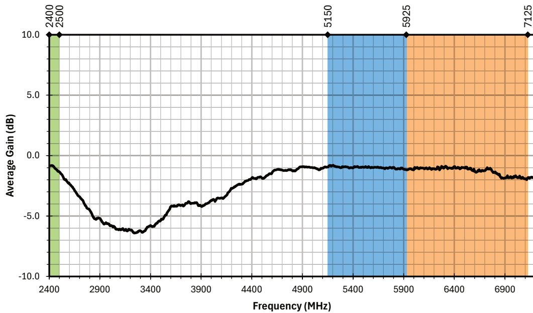
Figure 5. AC11005 Antenna Average Gain
