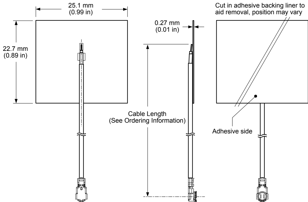
Figure 1. AC11005 Antenna Dimensions
