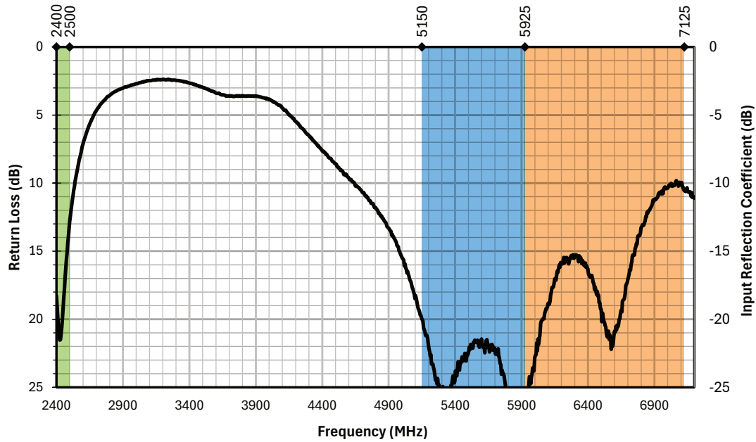
Figure 3. AC11005 Antenna Return Loss
