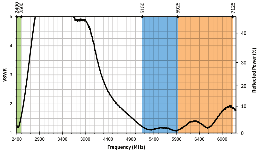
Figure 2. AC11005 Antenna VSWR
