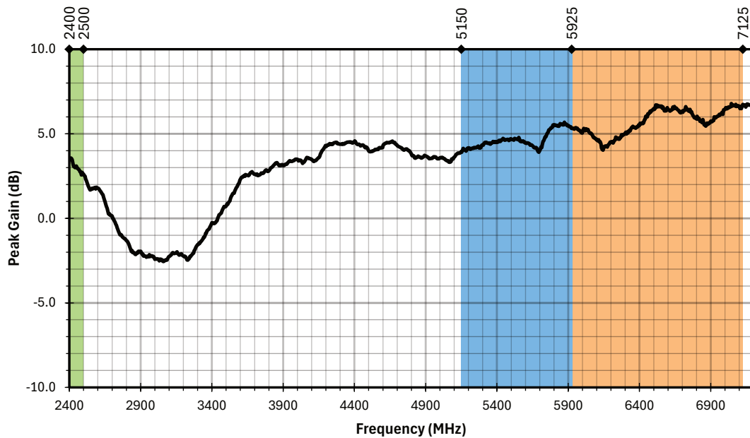
Figure 4. AC11005 Antenna Peak Gain
