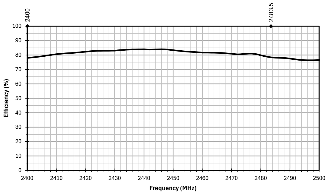
Figure 6. AC11501 Antenna Efficiency
