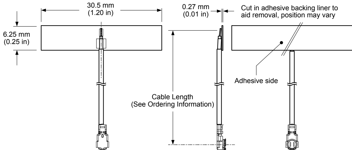
Figure 1. AC11501 Antenna Dimensions
