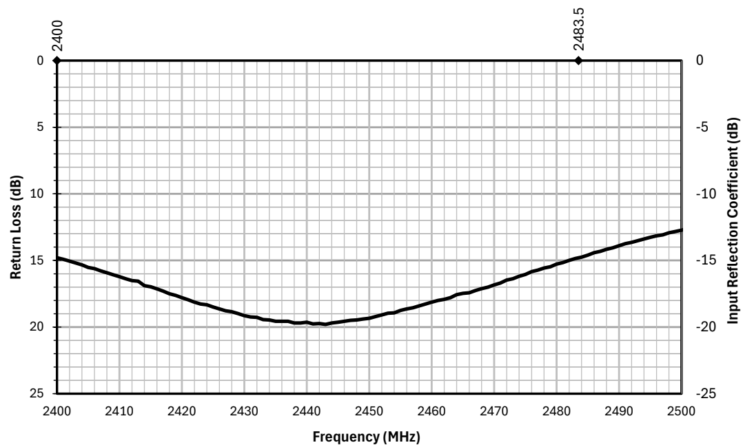
Figure 3. AC11501 Antenna Return Loss
