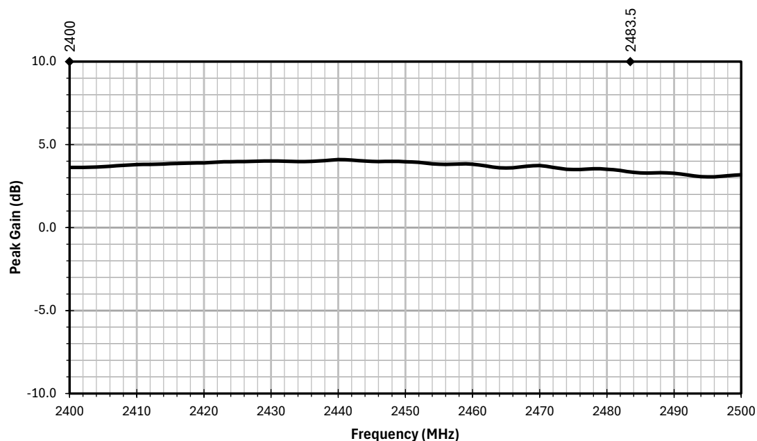
Figure 4. AC11501 Antenna Peak Gain
