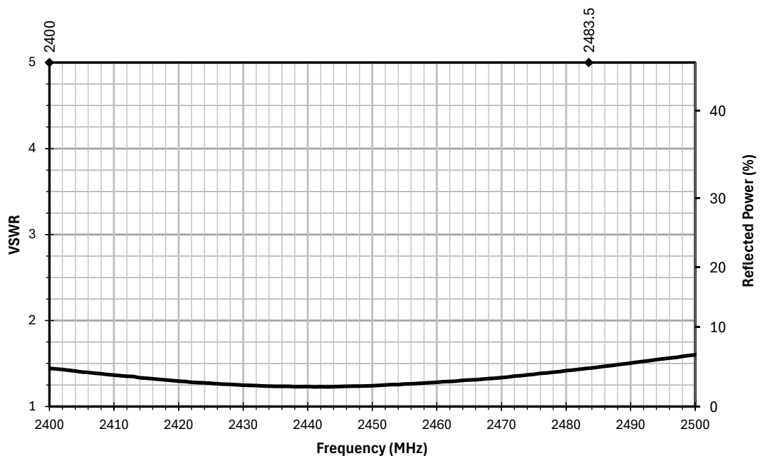
Figure 2. AC11501 Antenna VSWR
