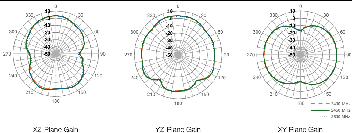
Figure 7. Radiation Patterns for the AC11501 Antenna
