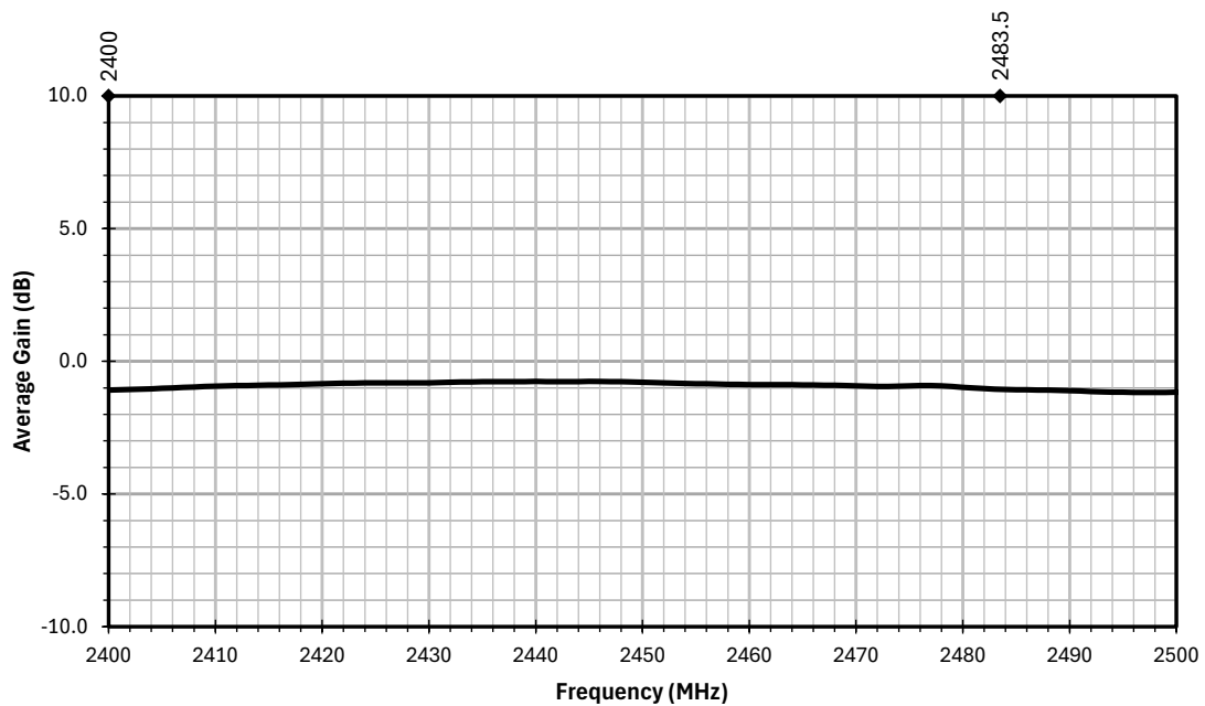
Figure 5. AC11501 Antenna Average Gain
