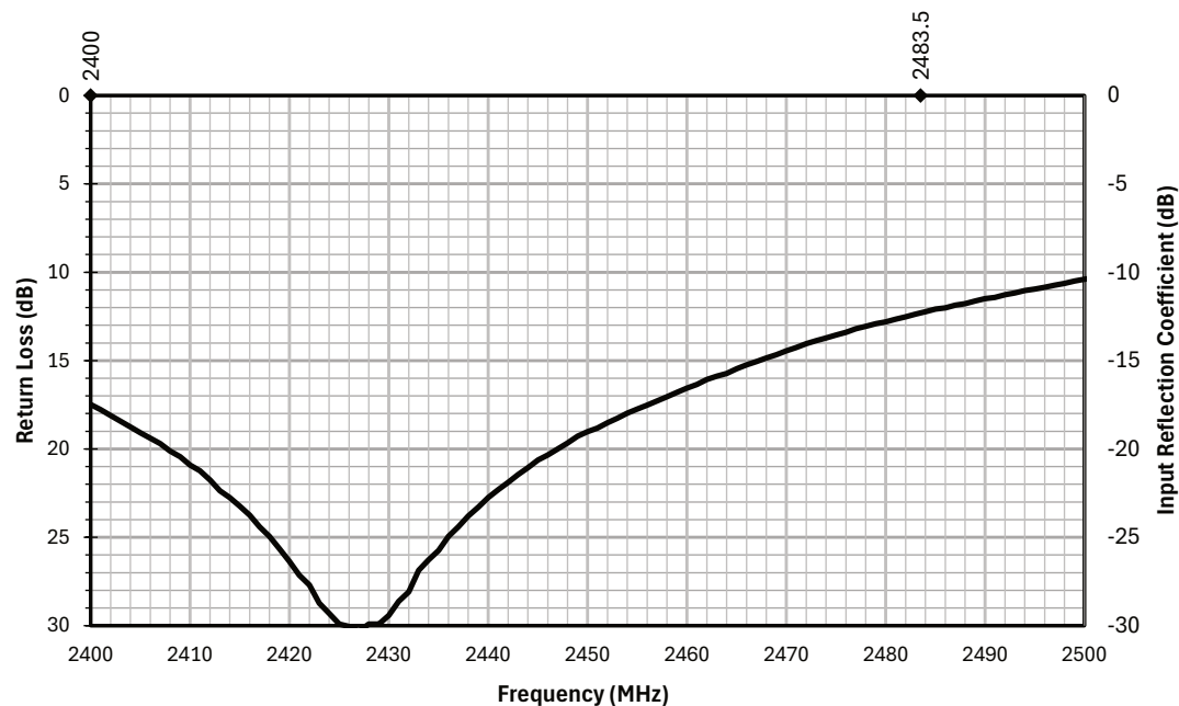
Figure 3. AC11503 Antenna Return Loss
