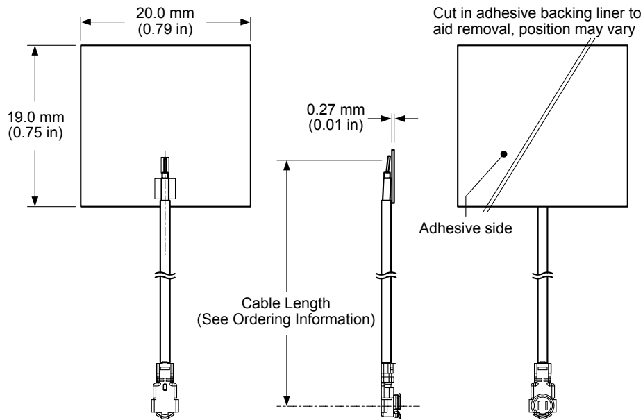
Figure 1. AC11503 Antenna Dimensions
