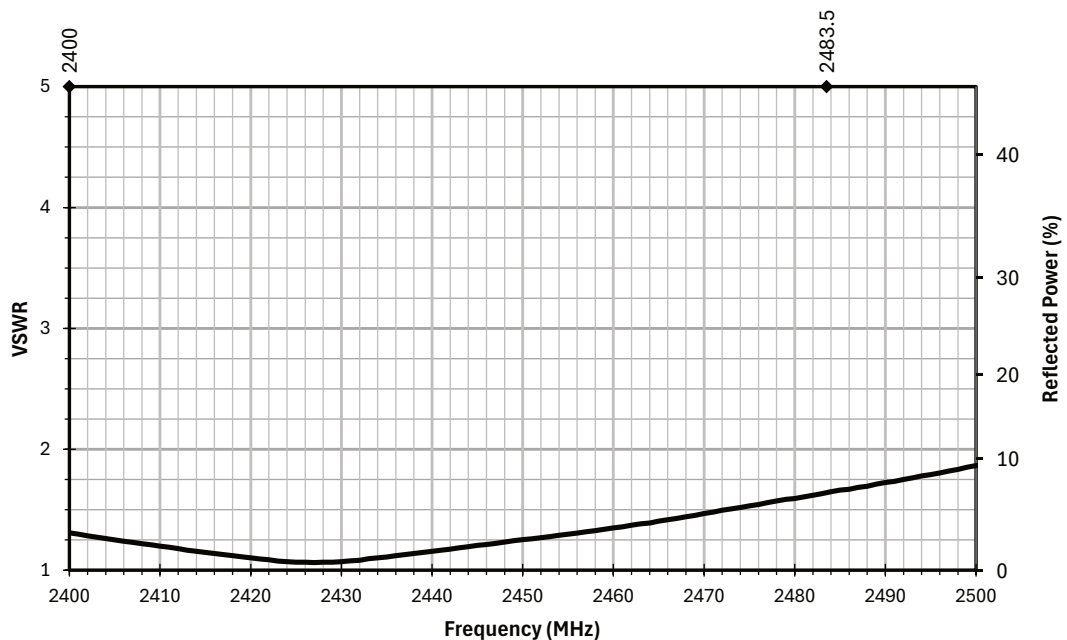
Figure 2. AC11503 Antenna VSWR
