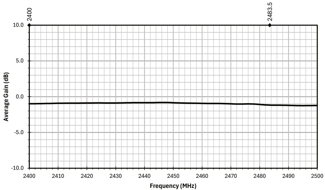
Figure 5. AC11503 Antenna Average Gain
