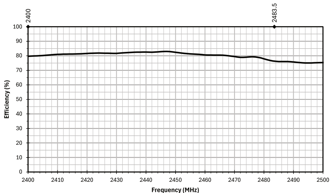
Figure 6. AC11503 Antenna Efficiency
