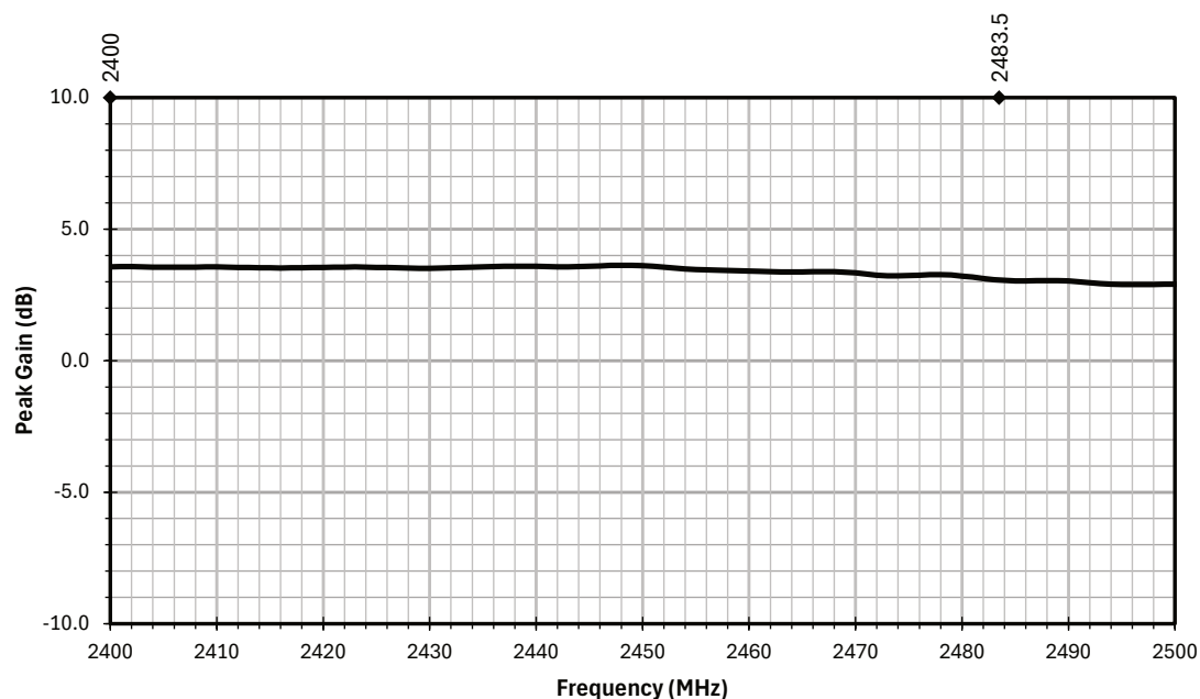
Figure 4. AC11503 Antenna Peak Gain
