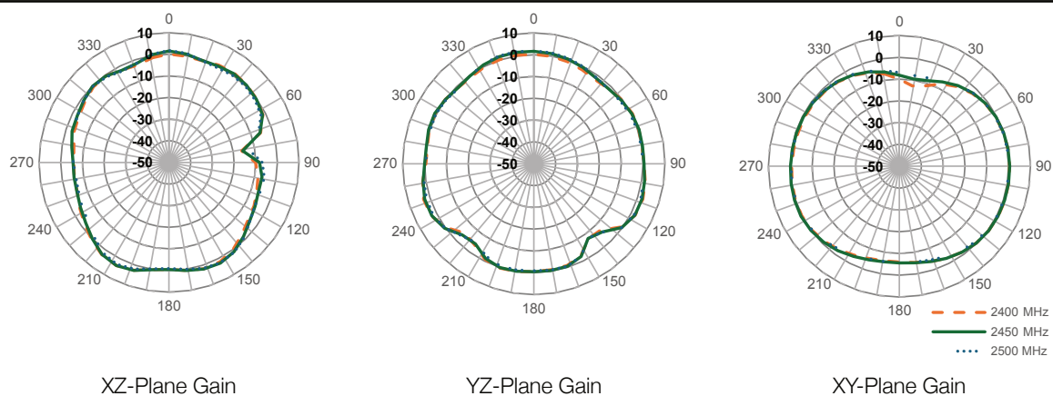
Figure 7. Radiation Patterns for the AC11503 Antenna
