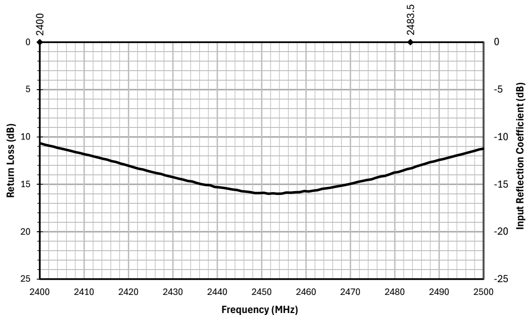
Figure 3. AC11504 Antenna Return Loss
