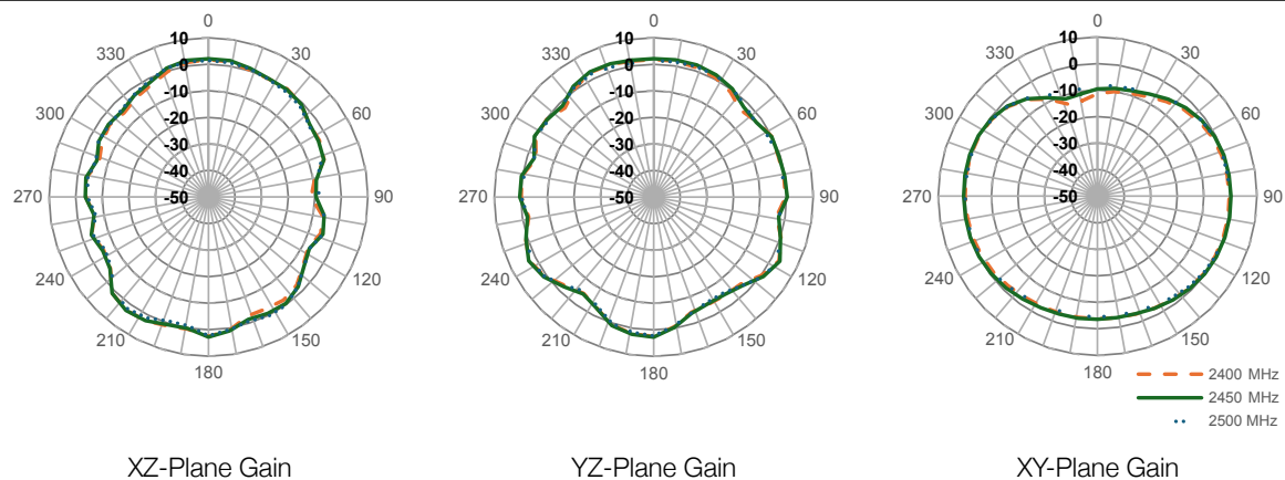
Figure 7. Radiation Patterns for the AC11504 Antenna
