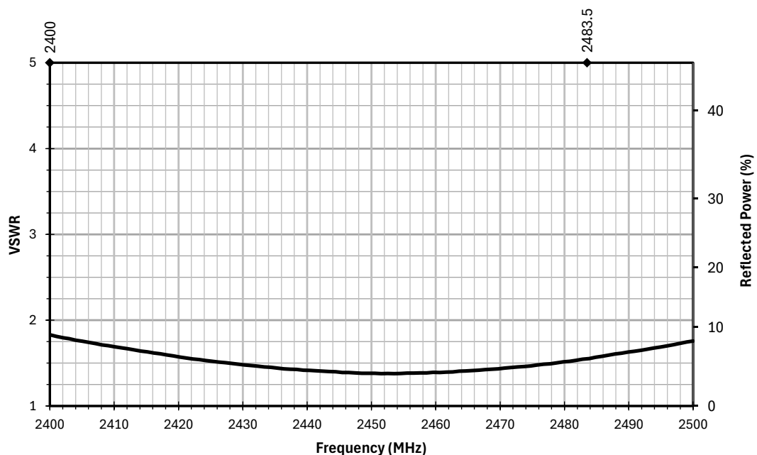
Figure 2. AC11504 Antenna VSWR
