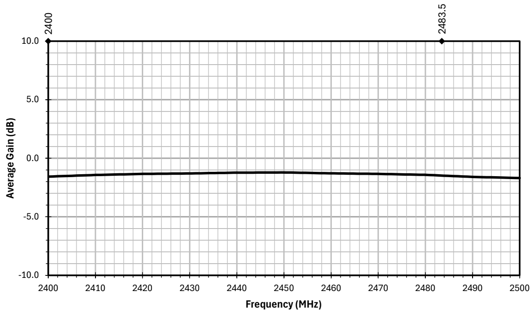
Figure 5. AC11504 Antenna Average Gain
