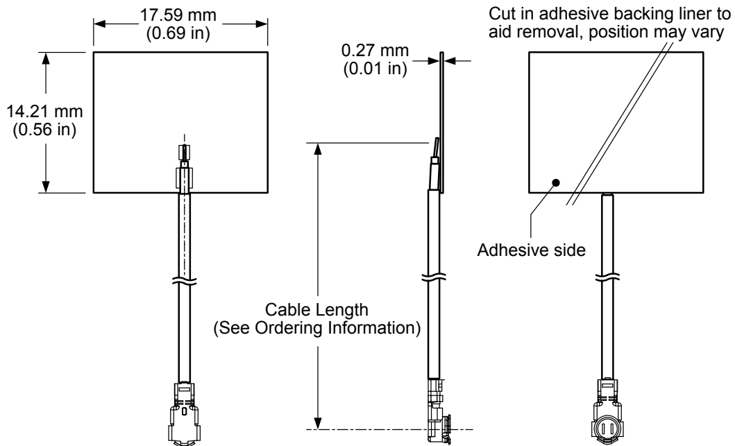
Figure 1. AC11504 Antenna Dimensions
