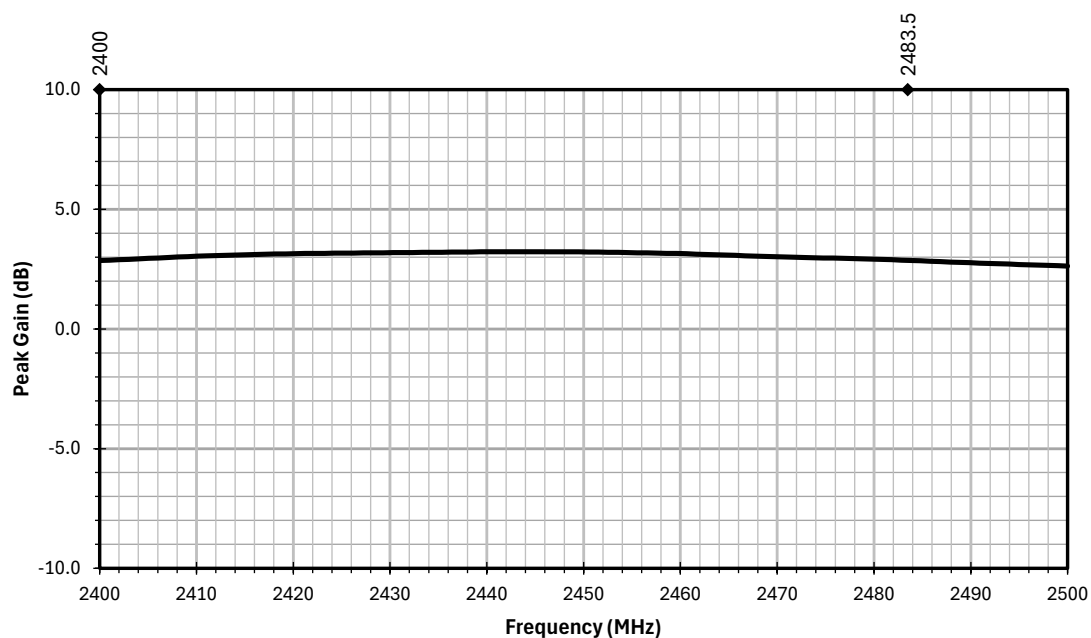
Figure 4. AC11504 Antenna Peak Gain
