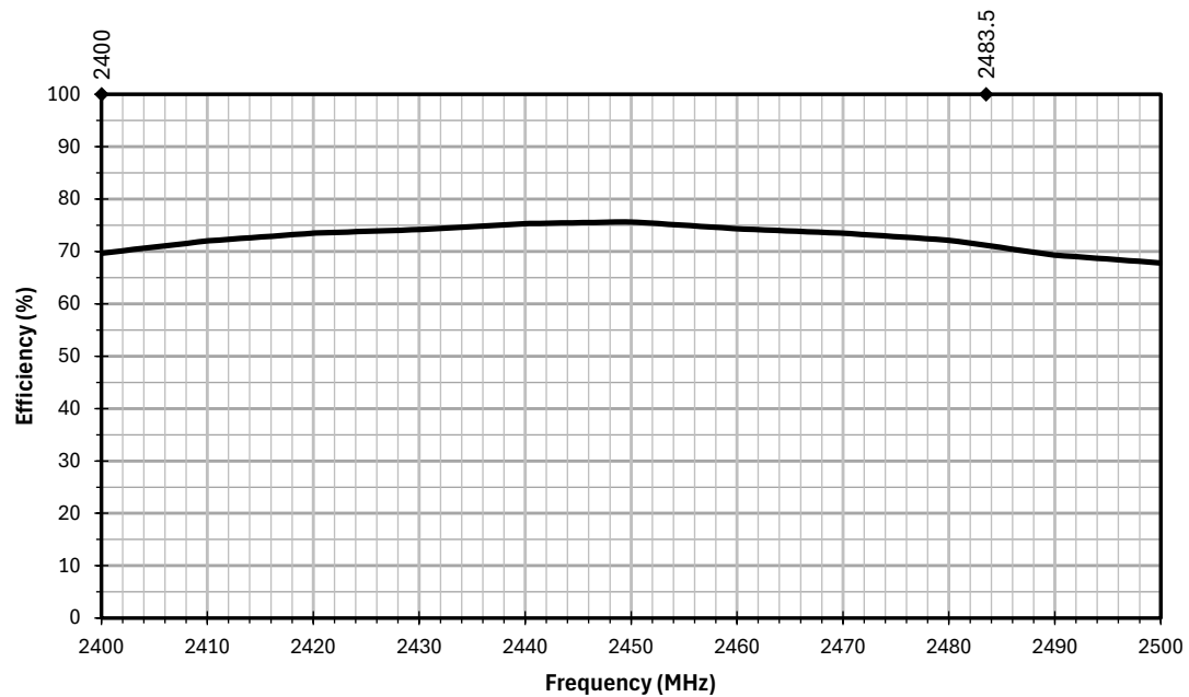
Figure 6. AC11504 Antenna Efficiency
