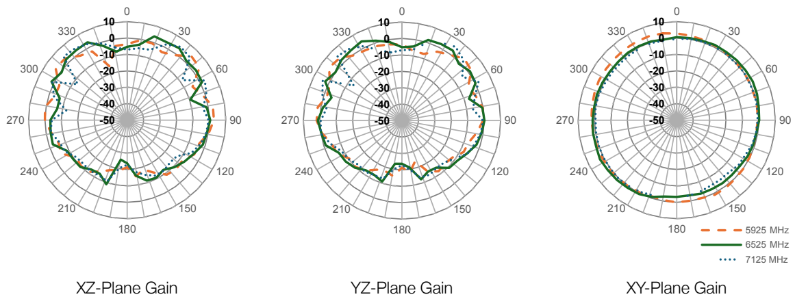
Figure 10. Radiation Patterns for AC15001 Antenna on Ground Plane
