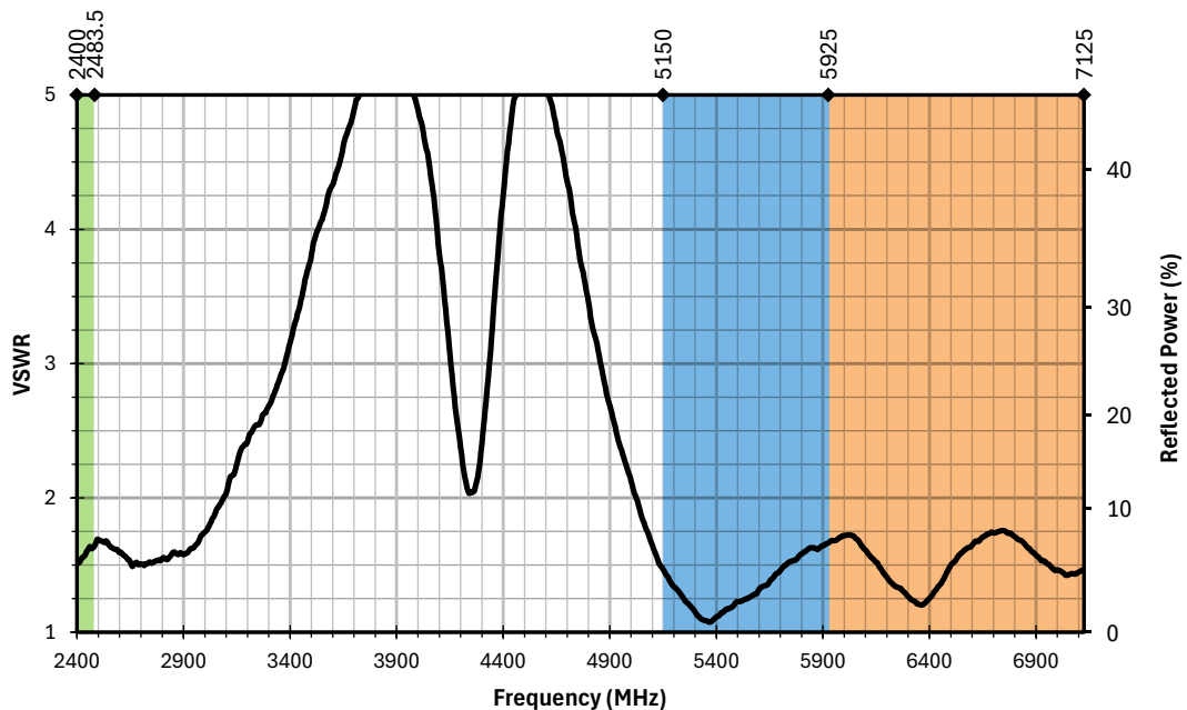
Figure 5. AC15001 Antenna VSWR on Ground Plane
