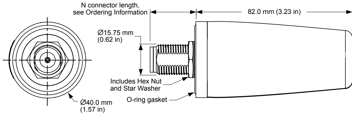
Figure 1. AC15001 Antenna Dimensions
