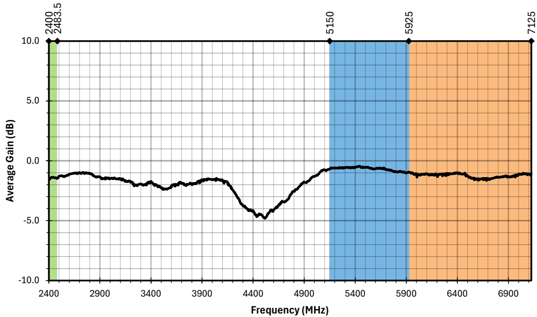
Figure 15. AC15001 Antenna Average Gain, Free Space
