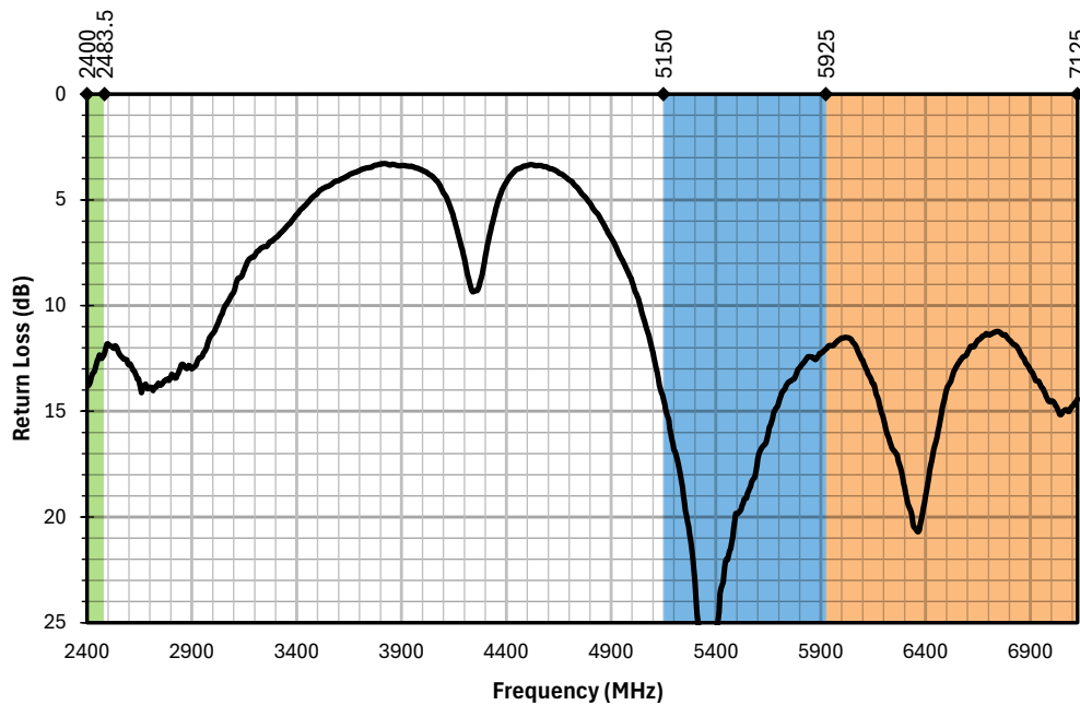
Figure 6. AC15001 Antenna Return Loss on Ground Plane
