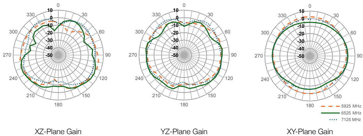
Figure 17. Radiation Patterns for AC15001 Antenna in Free Space
