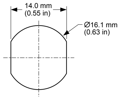
Figure 2. AC15001-NJ Antenna Mounting Dimensions
