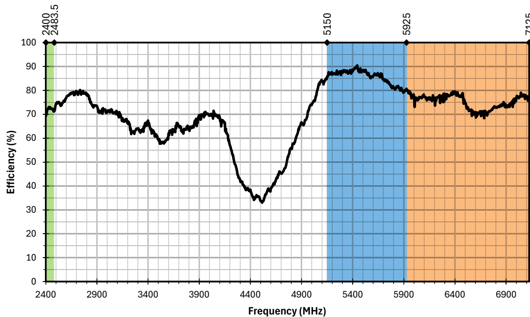
Figure 16. AC15001 Antenna Efficiency, Free Space
