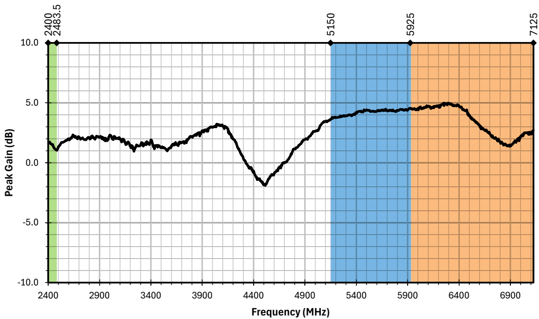
Figure 14. AC15001 Antenna Peak Gain, Free Space
