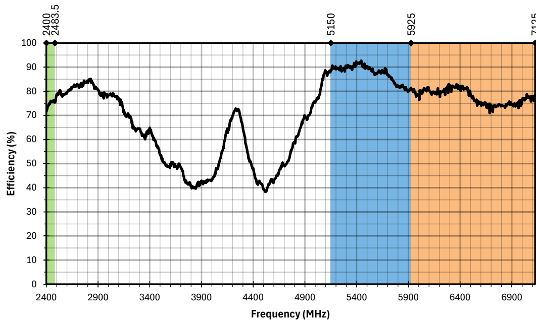
Figure 9. AC15001 Antenna Efficiency on Ground Plane
