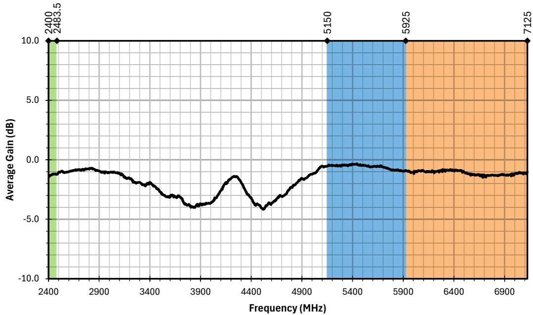
Figure 8. AC15001 Antenna Average Gain on Ground Plane
