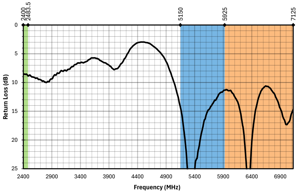
Figure 13. AC15001 Antenna Return Loss, Free Space
