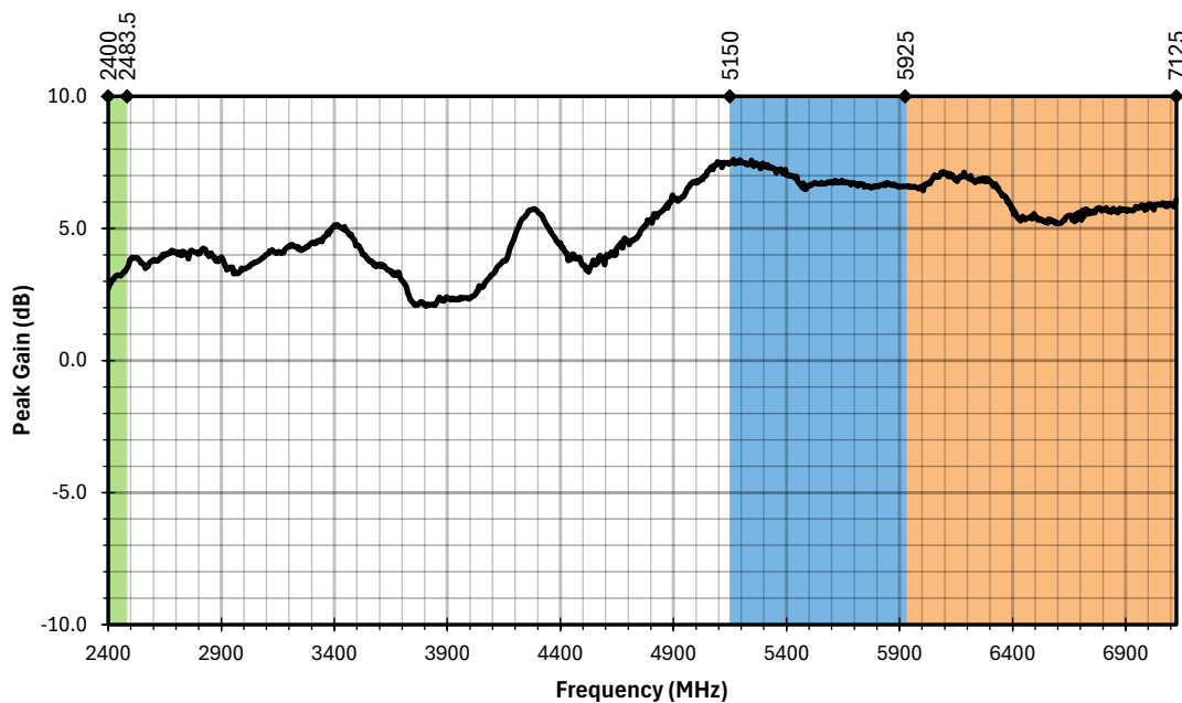
Figure 7. AC15001 Antenna Peak Gain on Ground Plane
