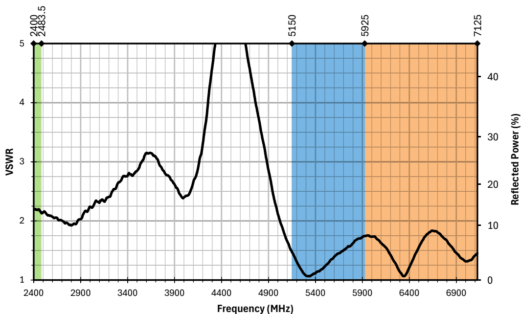
Figure 12. AC15001 Antenna VSWR, Free Space
