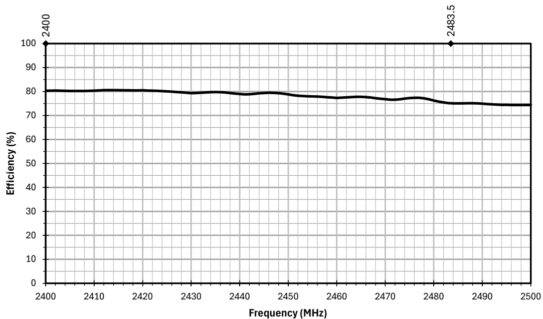
Figure 16. AC15101 Antenna Efficiency, Free Space
