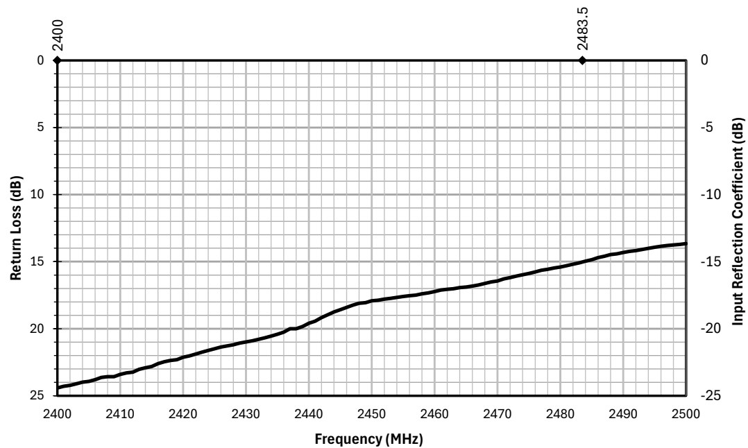
Figure 13. AC15101 Antenna Return Loss, Free Space
