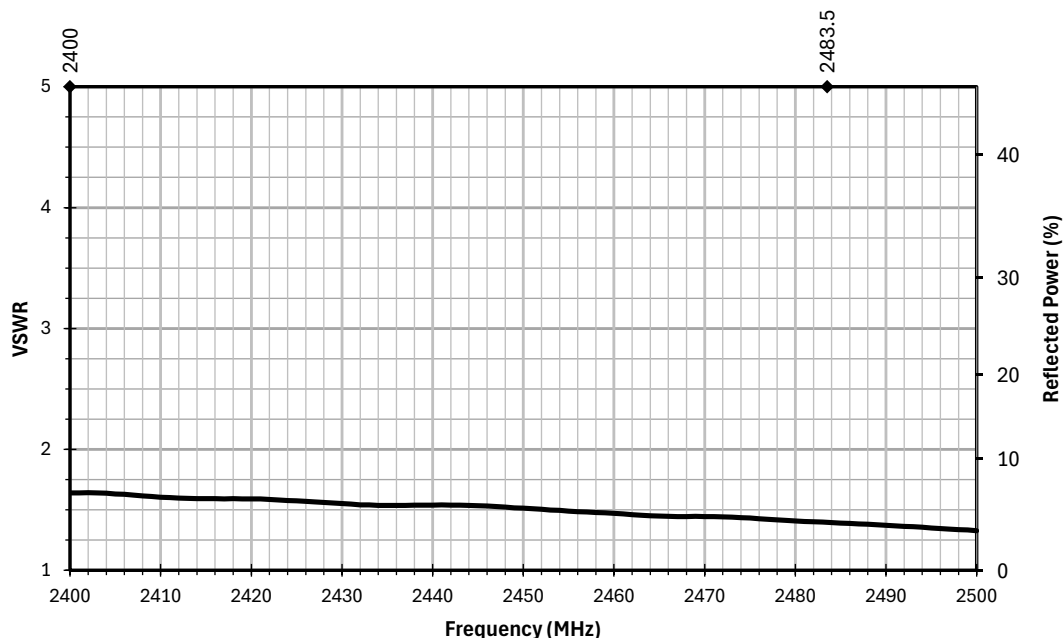
Figure 5. AC15101 Antenna VSWR on Ground Plane
