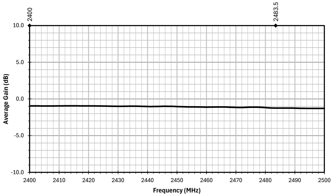
Figure 15. AC15101 Antenna Average Gain, Free Space
