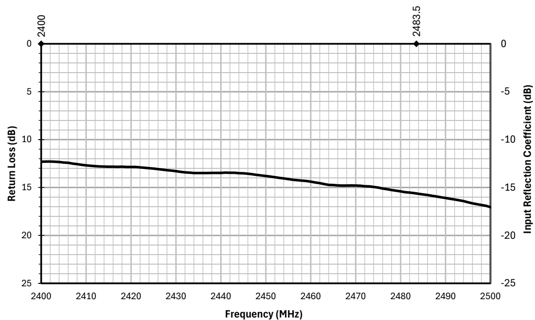
Figure 6. AC15101 Antenna Return Loss on Ground Plane
