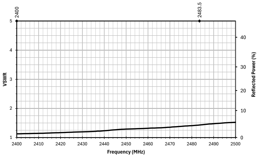
Figure 12. AC15101 Antenna VSWR, Free Space
