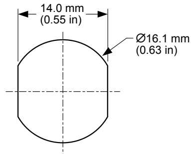
Figure 2. AC15101-NJ Antenna Mounting Dimensions
