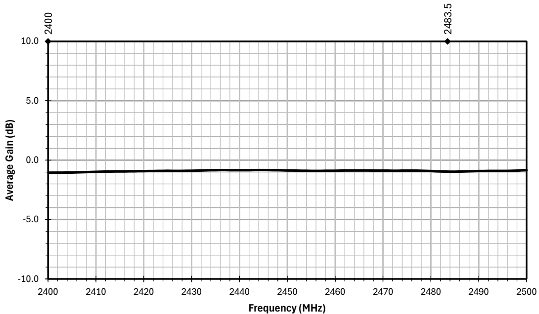
Figure 8. AC15101 Antenna Average Gain on Ground Plane
