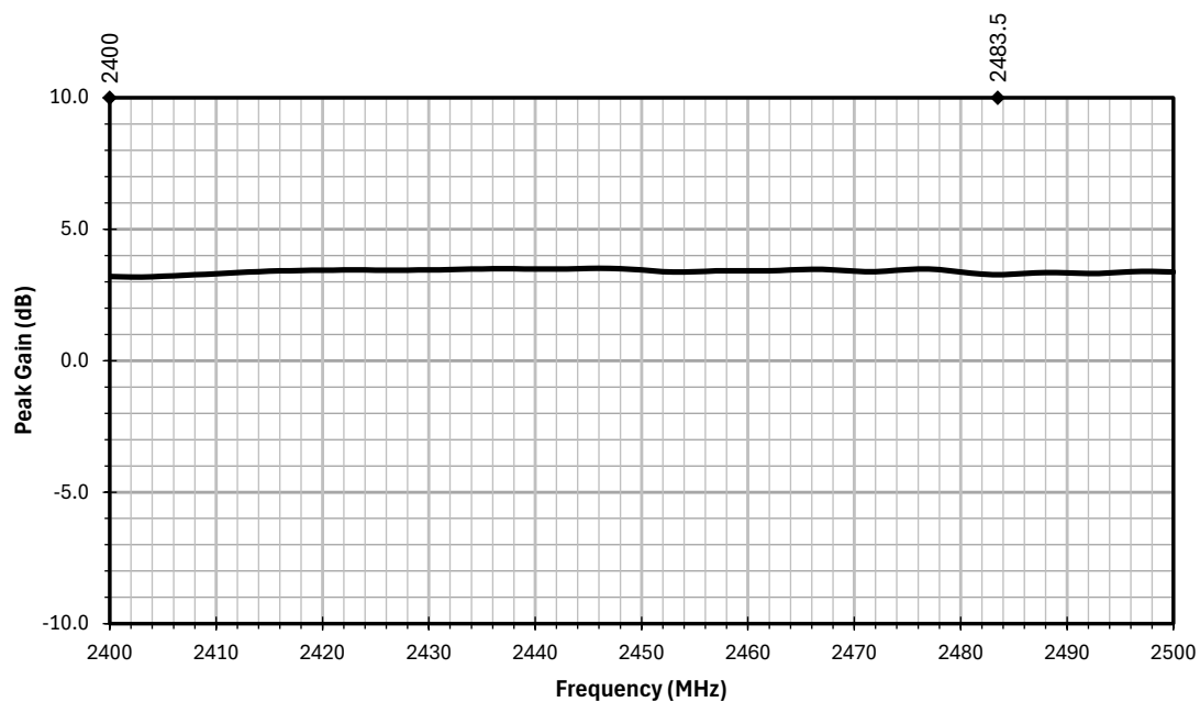
Figure 7. AC15101 Antenna Peak Gain on Ground Plane
