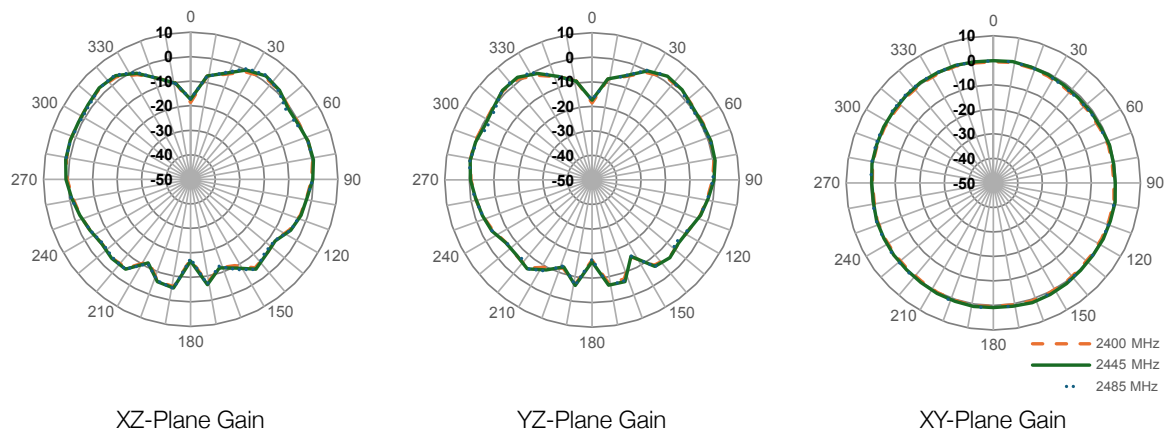
Figure 10. Radiation Patterns for AC15101 Antenna on Ground Plane
