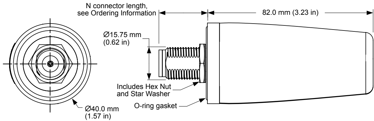
Figure 1. AC15101 Antenna Dimensions
