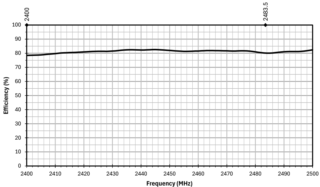
Figure 9. AC15101 Antenna Efficiency on Ground Plane
