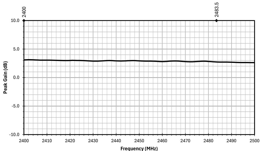
Figure 14. AC15101 Antenna Peak Gain, Free Space
