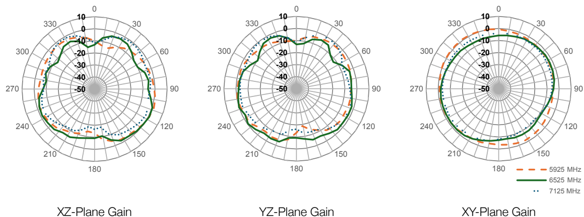
Figure 17. Radiation Patterns for AC17001 Antenna in Free Space
