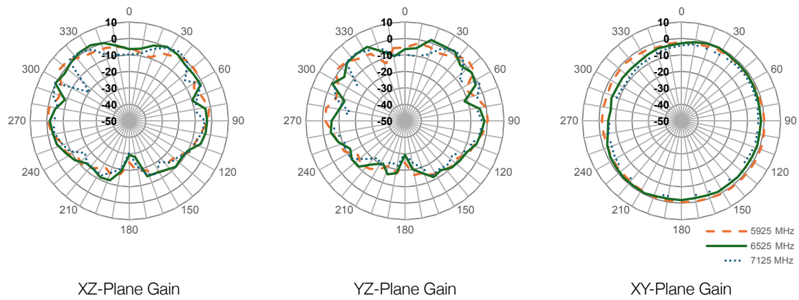
Figure 10. Radiation Patterns for AC17001 Antenna on Ground Plane
