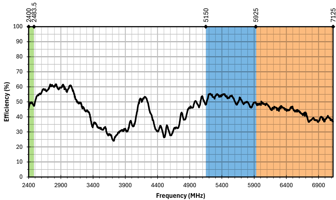
Figure 9. AC17001 Antenna Efficiency on Ground Plane
