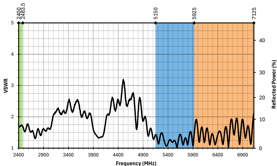
Figure 12. AC17001 Antenna VSWR, Free Space
