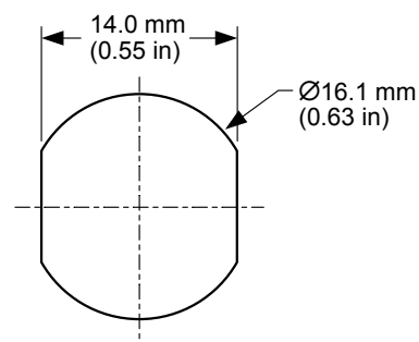
Figure 2. AC17001 Antenna Mounting Dimensions
