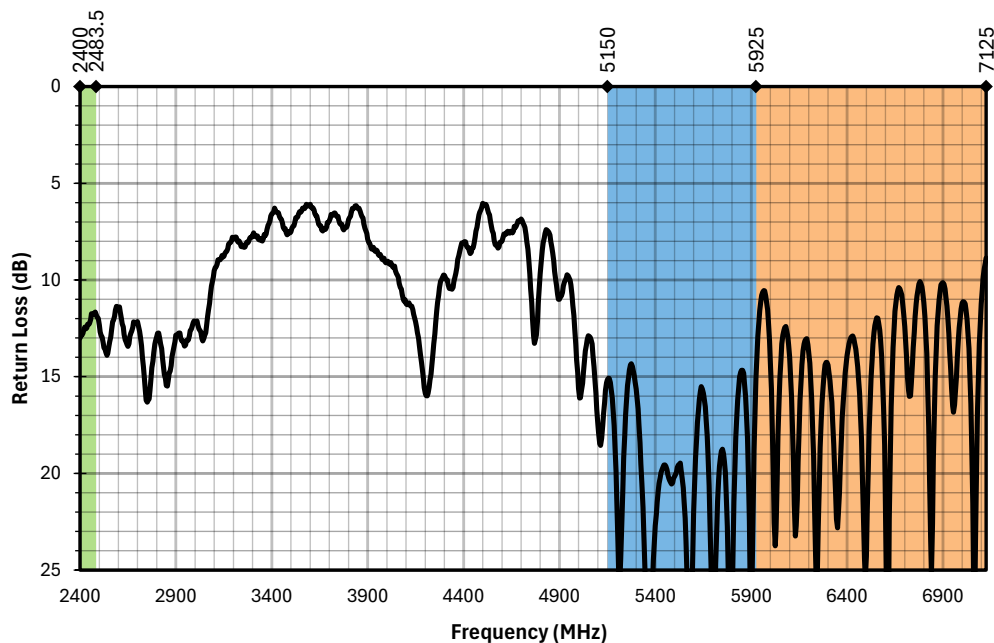
Figure 6. AC17001 Antenna Return Loss on Ground Plane
