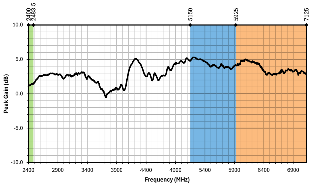
Figure 7. AC17001 Antenna Peak Gain on Ground Plane
