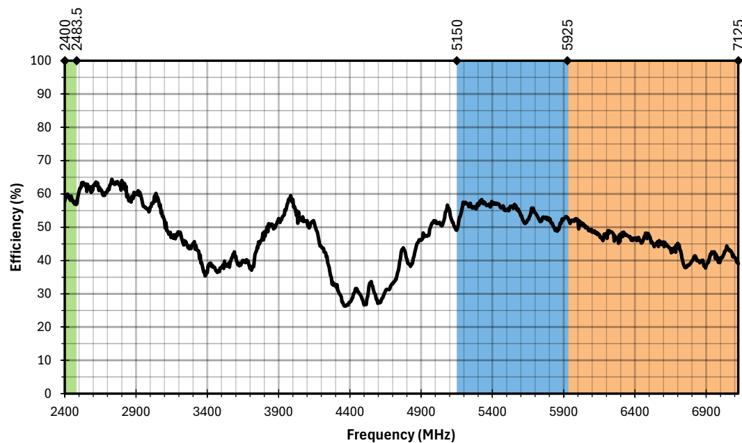
Figure 16. AC17001 Antenna Efficiency, Free Space
