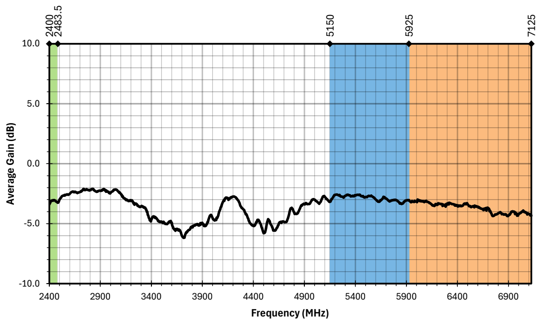
Figure 8. AC17001 Antenna Average Gain on Ground Plane
