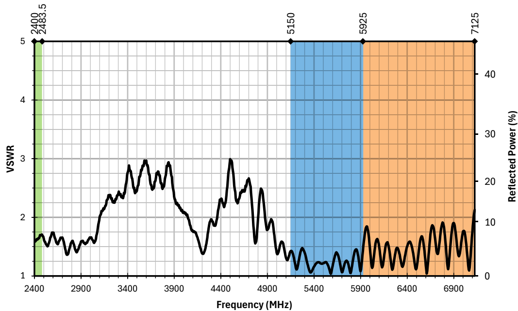
Figure 5. AC17001 Antenna VSWR on Ground Plane
