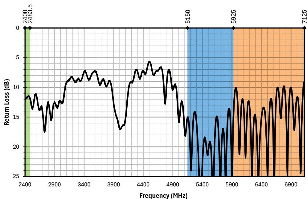
Figure 13. AC17001 Antenna Return Loss, Free Space
