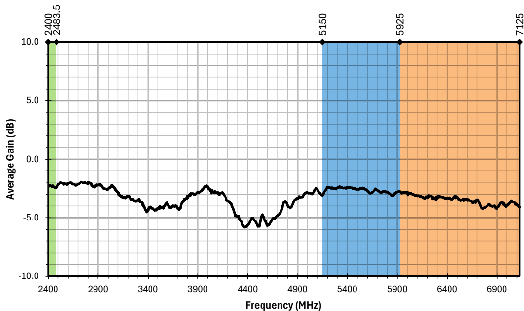
Figure 15. AC17001 Antenna Average Gain, Free Space
