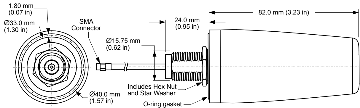
Figure 1. AC17001 Antenna Dimensions
