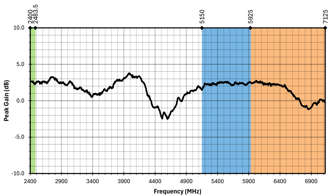
Figure 14. AC17001 Antenna Peak Gain, Free Space
