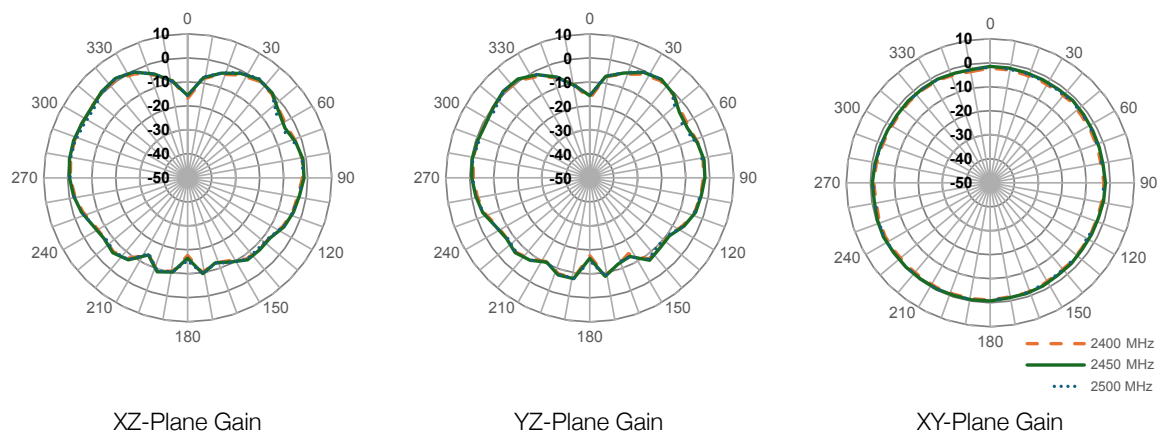
Figure 10. Radiation Patterns for AC17101 Antenna on Ground Plane
