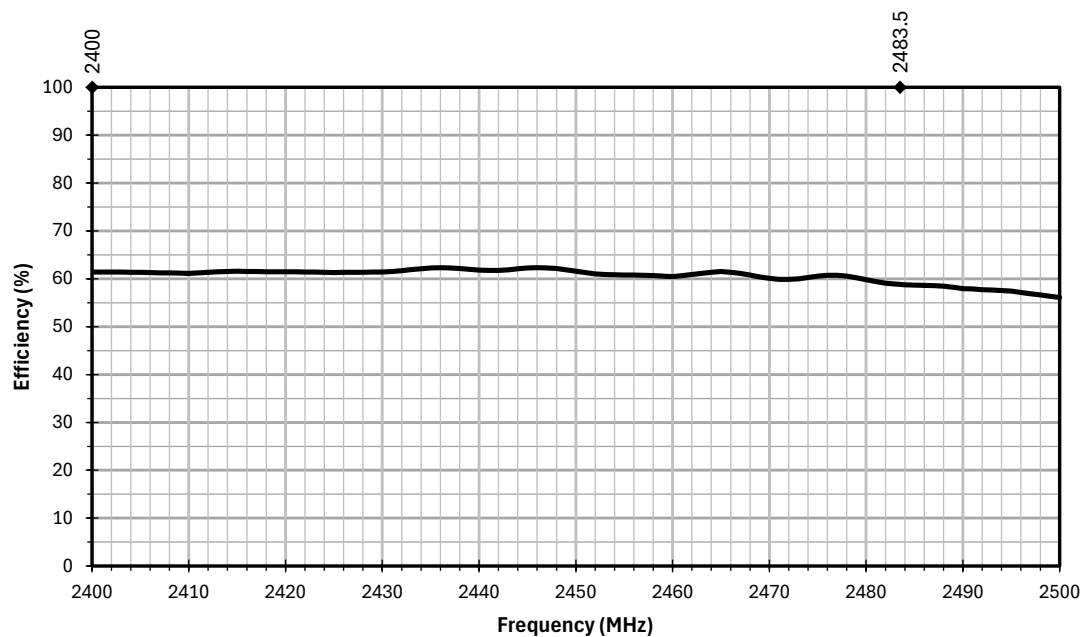
Figure 16. AC17101 Antenna Efficiency, Free Space
