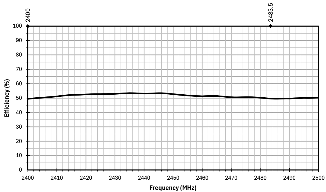
Figure 9. AC17101 Antenna Efficiency on Ground Plane
