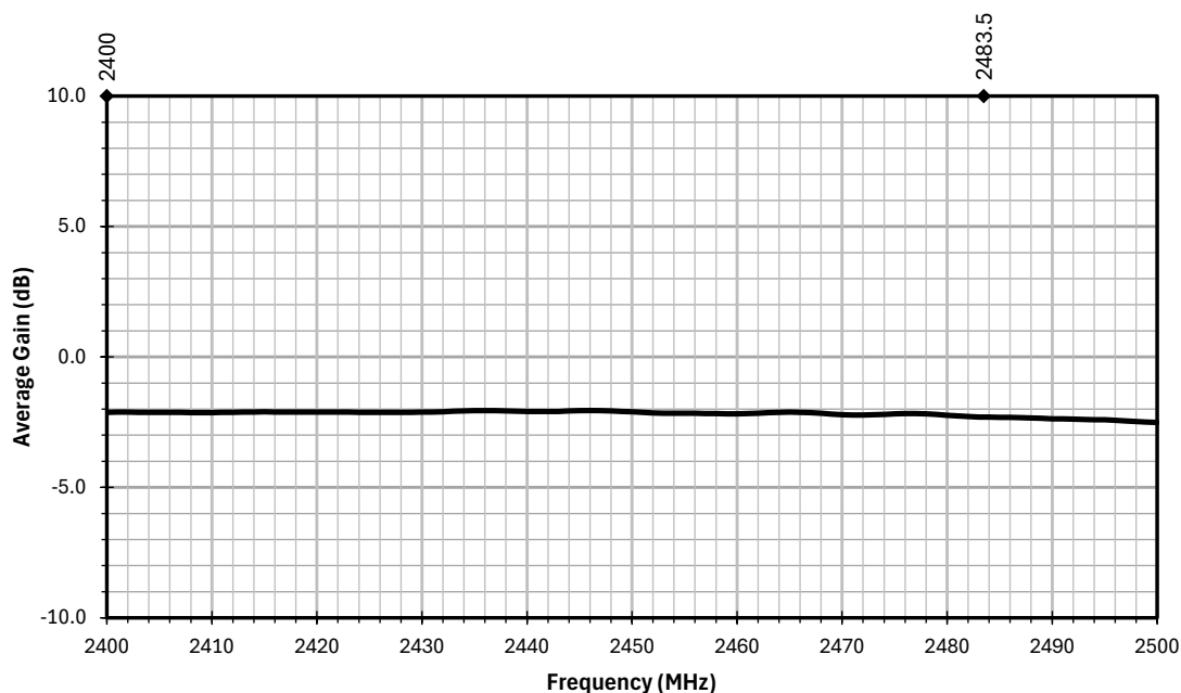
Figure 15. AC17101 Antenna Average Gain, Free Space
