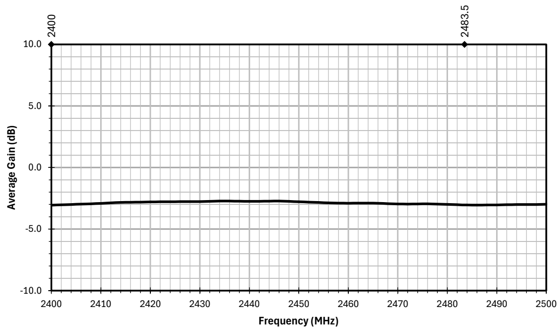
Figure 8. AC17101 Antenna Average Gain on Ground Plane
