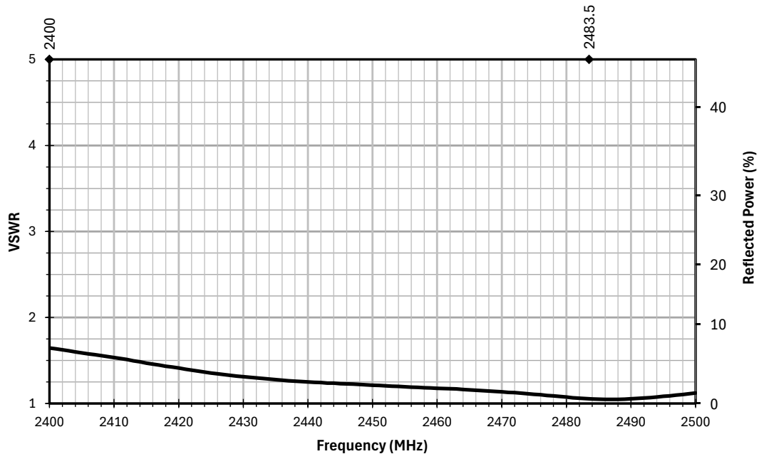
Figure 5. AC17101 Antenna VSWR on Ground Plane
