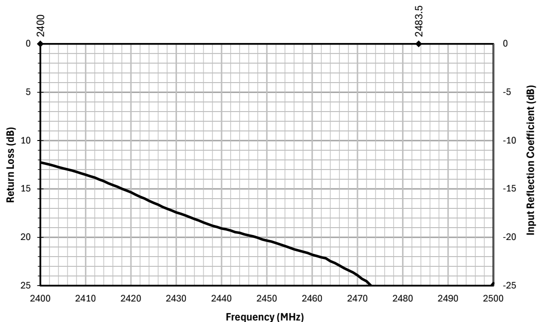
Figure 6. AC17101 Antenna Return Loss on Ground Plane
