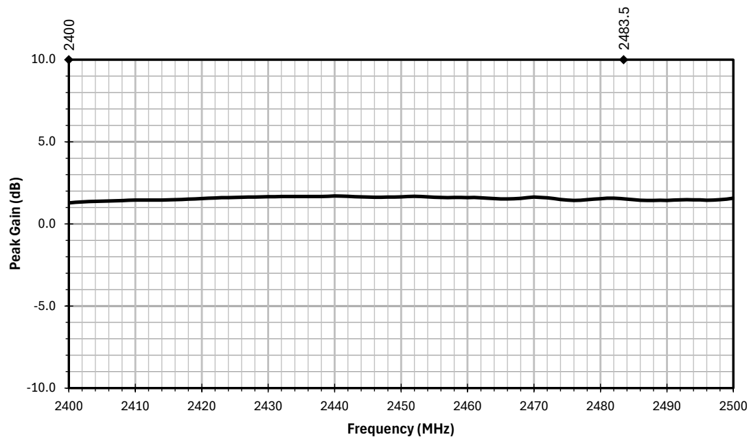
Figure 7. AC17101 Antenna Peak Gain on Ground Plane
