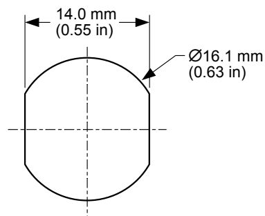
Figure 2. AC17101 Antenna Mounting Dimensions
