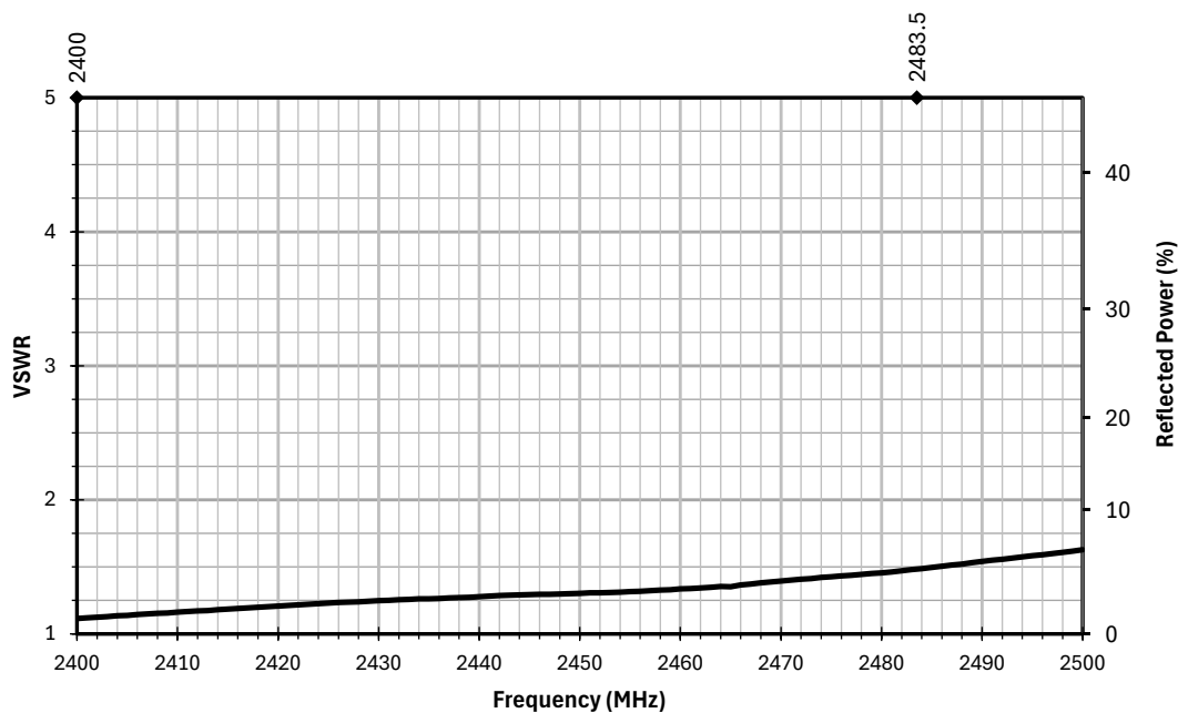
Figure 12. AC17101 Antenna VSWR, Free Space
