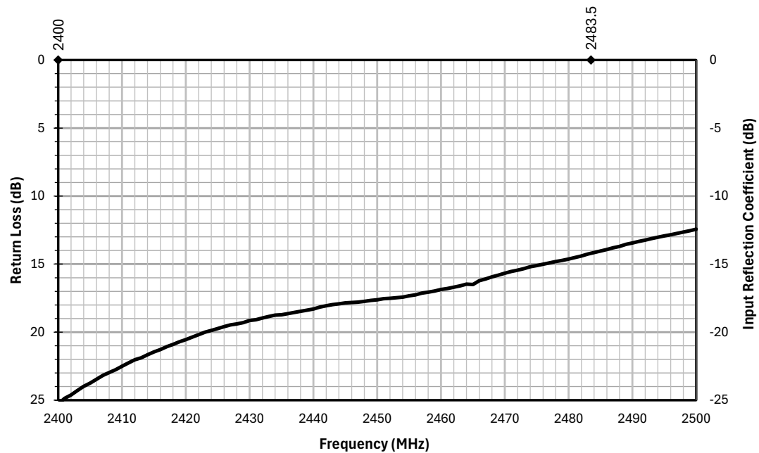
Figure 13. AC17101 Antenna Return Loss, Free Space
