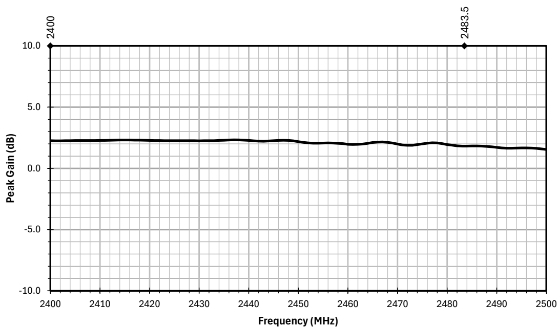
Figure 14. AC17101 Antenna Peak Gain, Free Space
