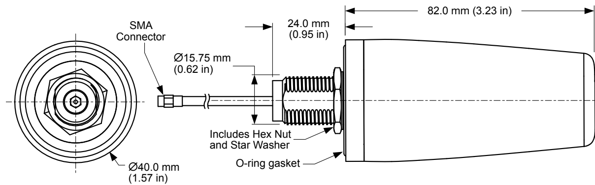
Figure 1. AC17101 Antenna Dimensions
