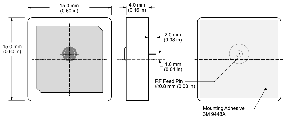
Figure 1. AC33154-1T Antenna Dimensions
