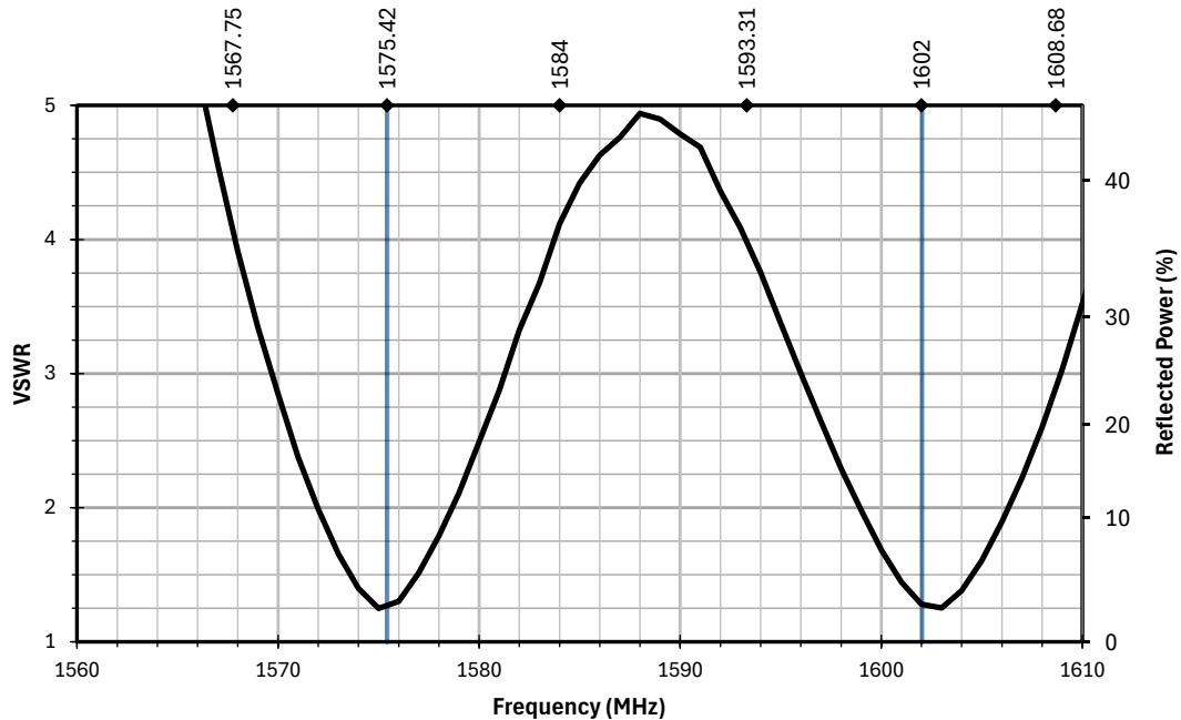
Figure 2. AC33154-1T Antenna VSWR with Frequency Band Highlights
