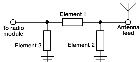
Figure 11. Recommended Matching Network
