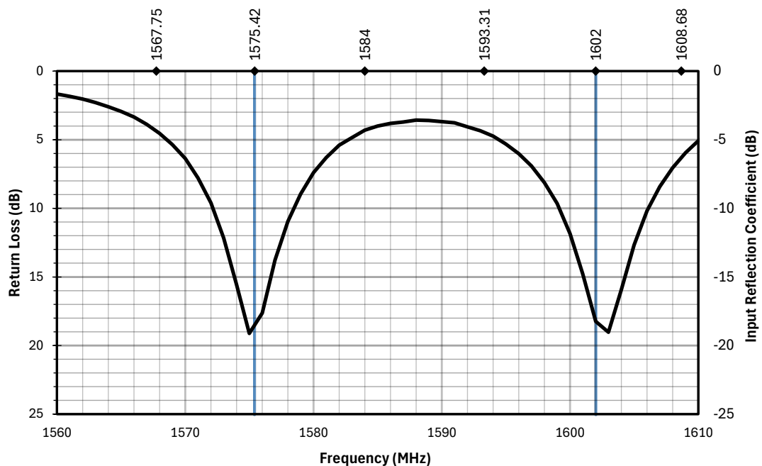
Figure 3. AC33154-1T Antenna Return Loss with Frequency Band Highlights
