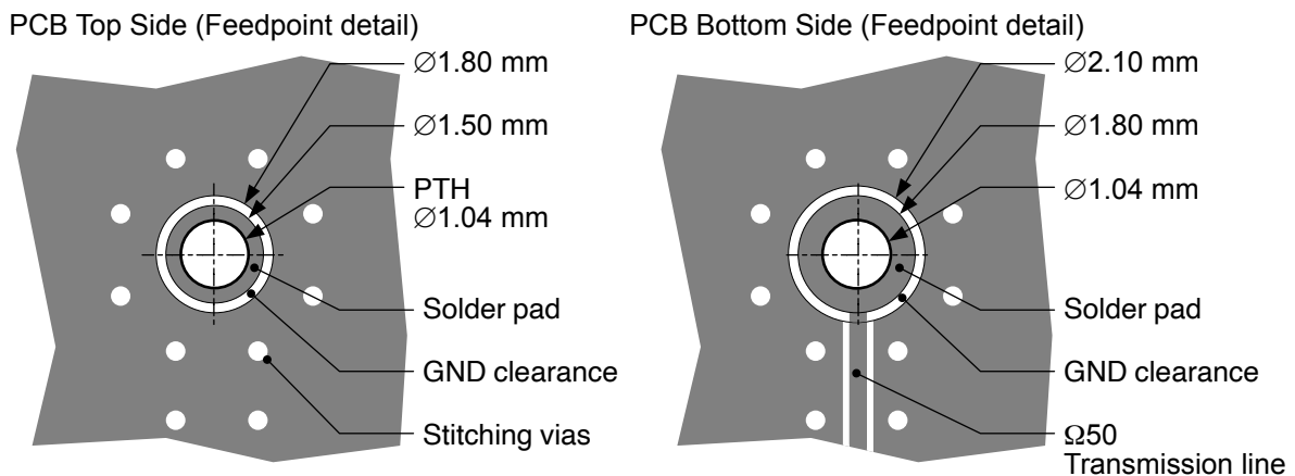
Figure 9. Recommended PCB Footprint for the AC33154-1T Antenna
