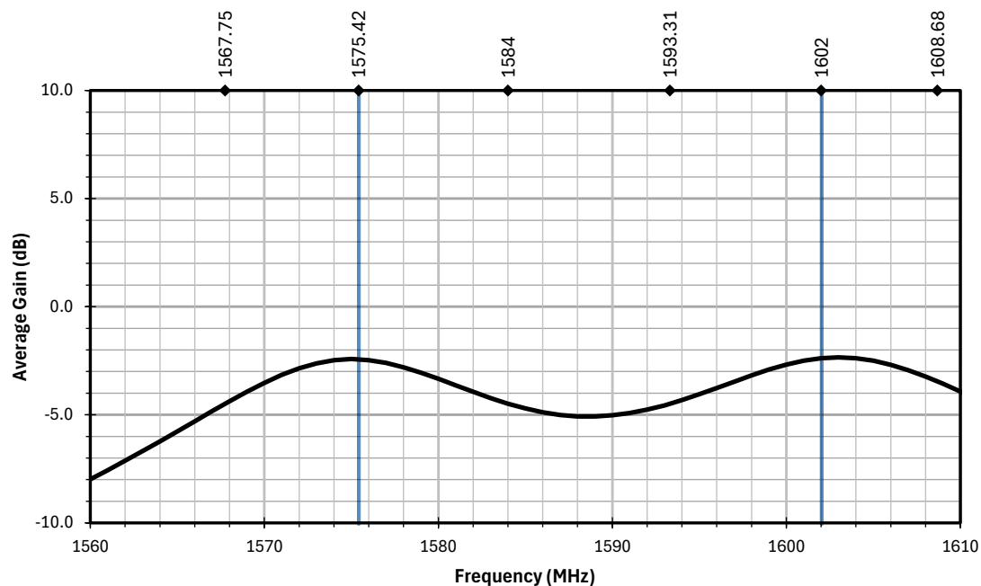
Figure 5. AC33154-1T Antenna Average Gain with Frequency Band Highlights
