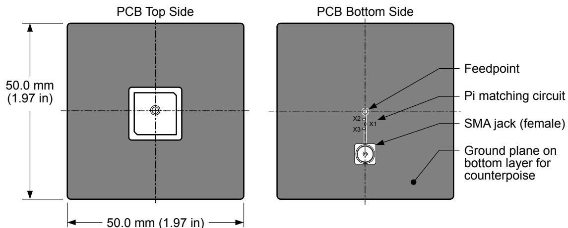
Figure 10. AC33154 Recommended Layout
