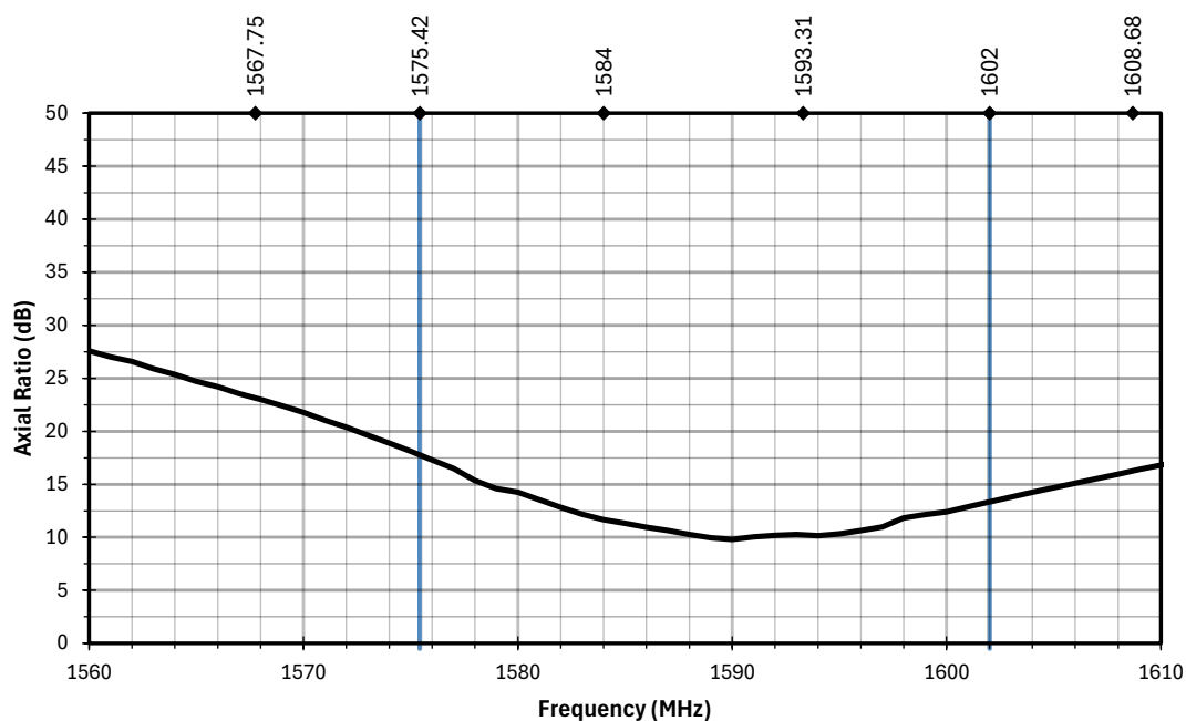
Figure 7. Axial Ratio for the AC33154-1T Antenna
