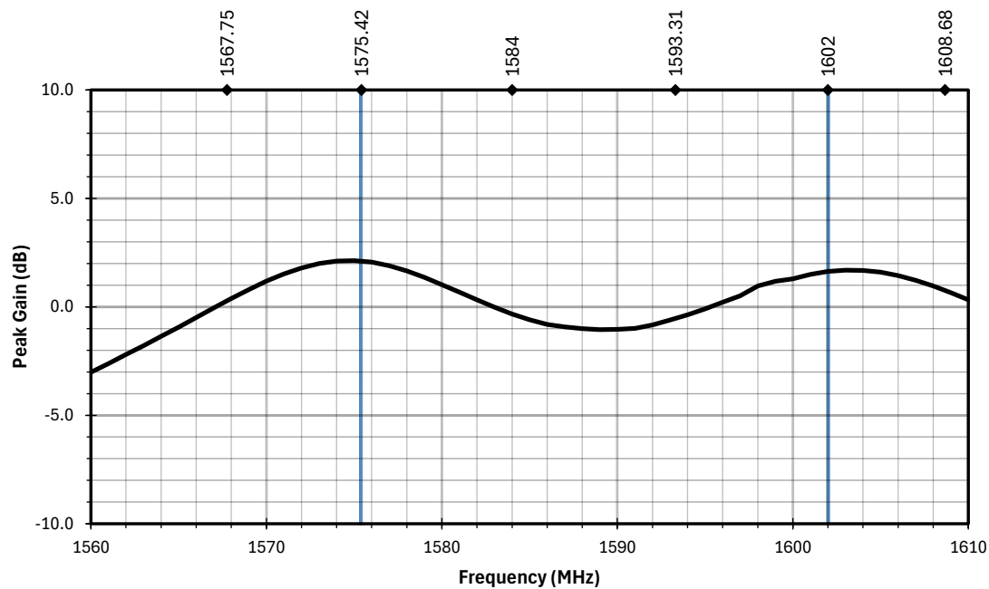
Figure 4. AC33154-1T Antenna Peak Gain with Frequency Band Highlights
