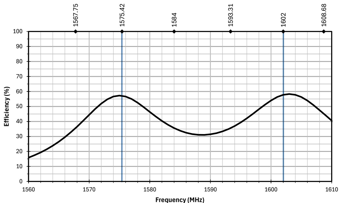
Figure 6. AC33154-1T Antenna Efficiency with Frequency Band Highlights
