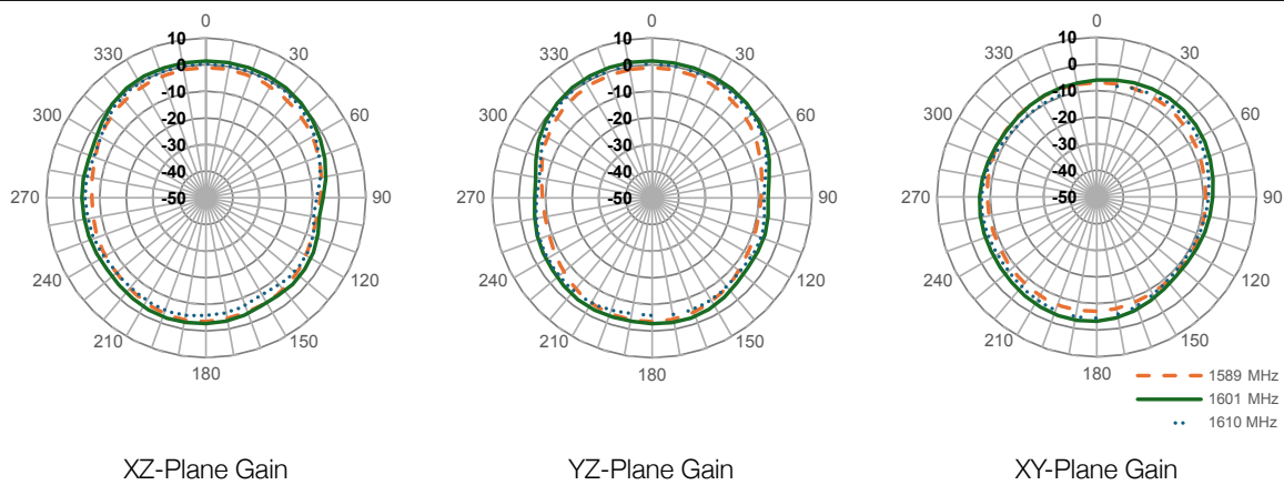
Figure 8. Radiation Patterns for AC33154-1T Antenna
