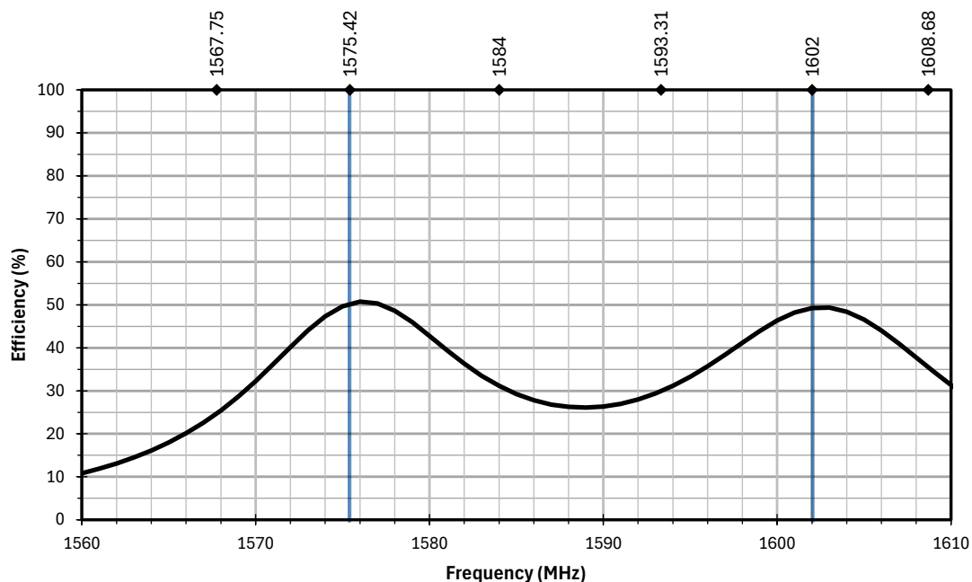
Figure 6. AC33182-1T Antenna Efficiency with Frequency Band Highlights
