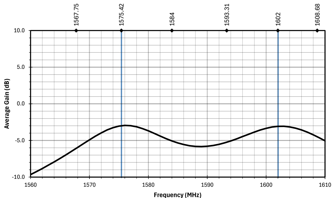
Figure 5. AC33182-1T Antenna Average Gain with Frequency Band Highlights
