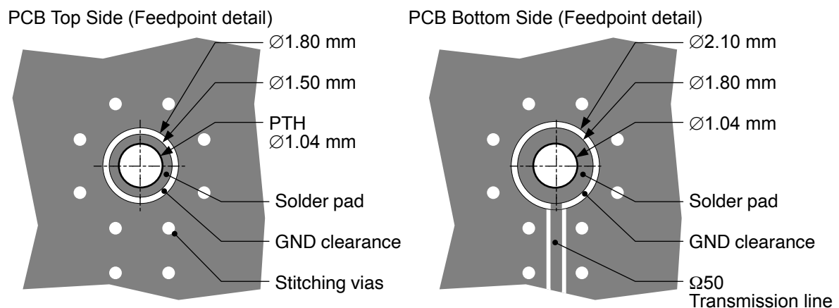
Figure 9. Recommended PCB Footprint for the AC33182-1T Antenna
