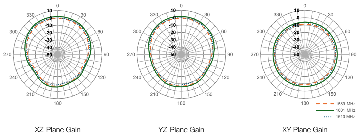
Figure 8. Radiation Patterns for AC33182-1T Antenna
