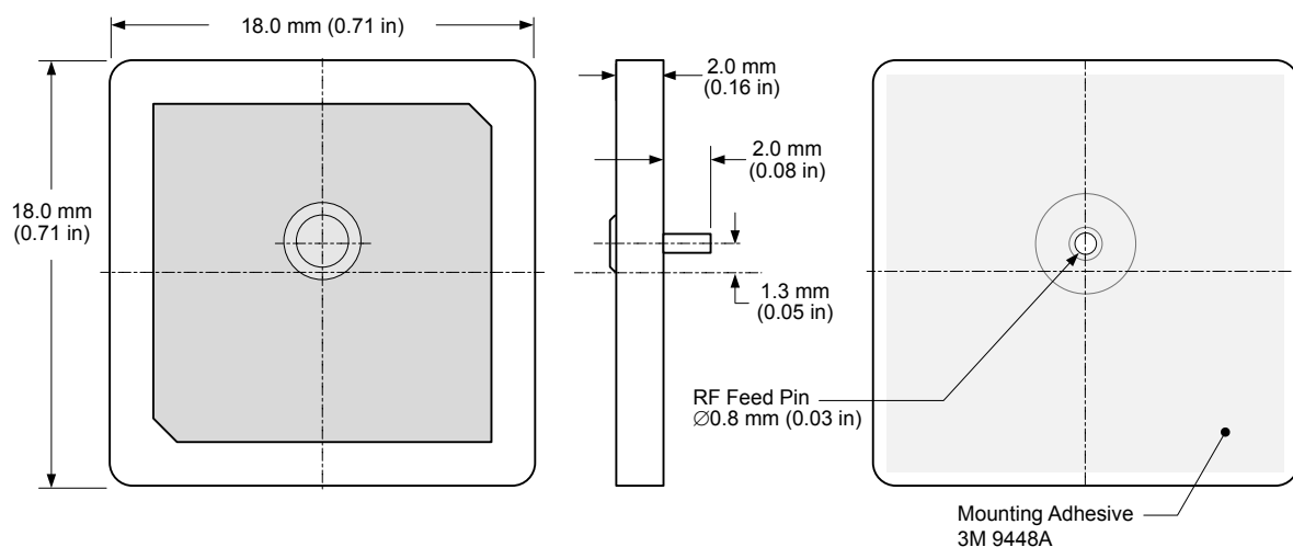
Figure 1. AC33182-1T Antenna Dimensions
