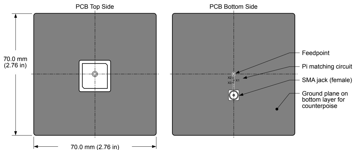
Figure 10. AC33182 Recommended Layout
