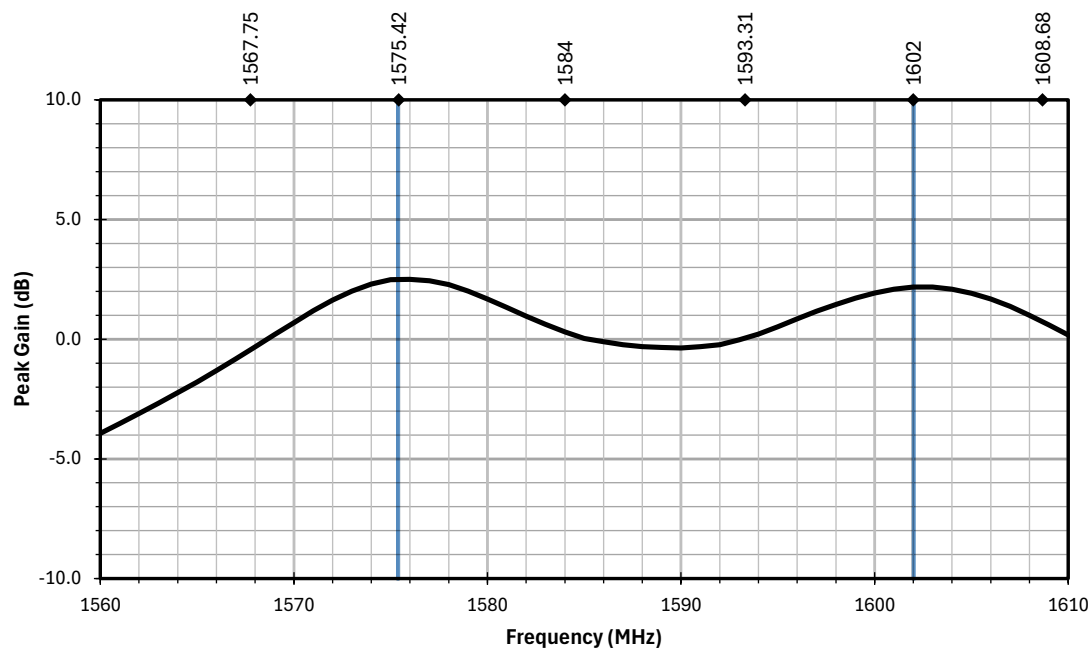
Figure 4. AC33182-1T Antenna Peak Gain with Frequency Band Highlights
