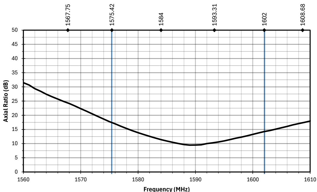
Figure 7. Axial Ratio for the AC33182-1T Antenna
