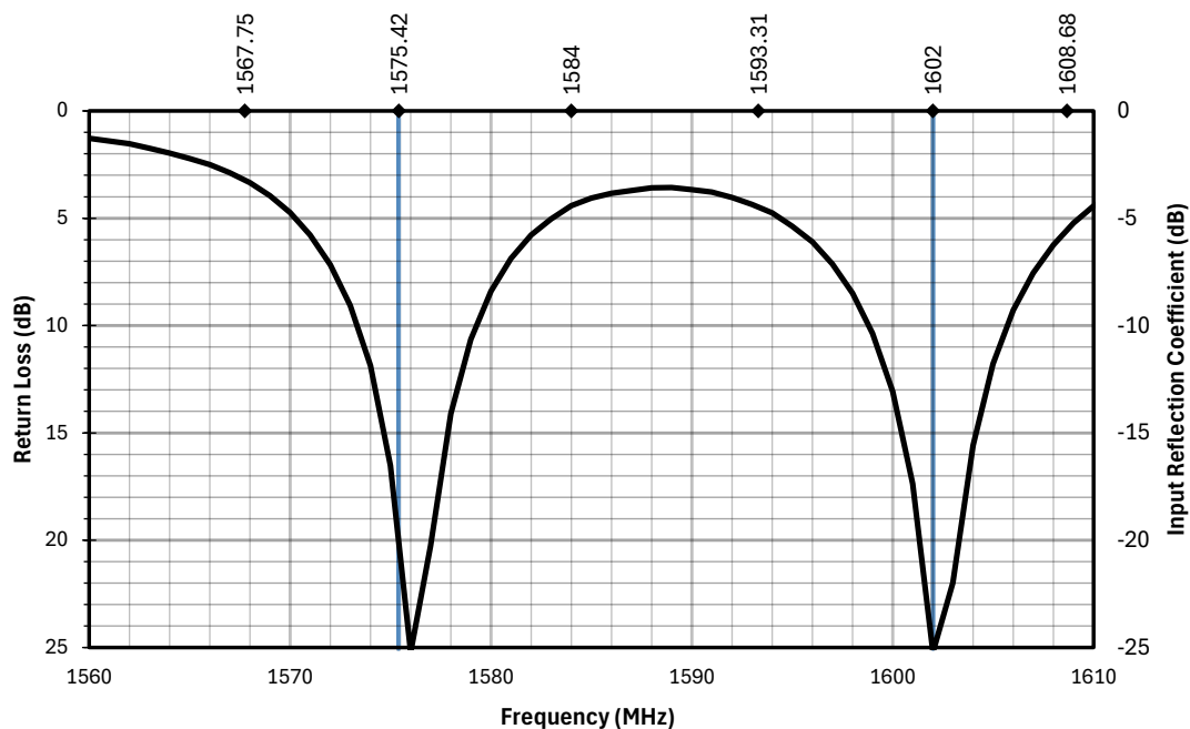
Figure 3. AC33182-1T Antenna Return Loss with Frequency Band Highlights
