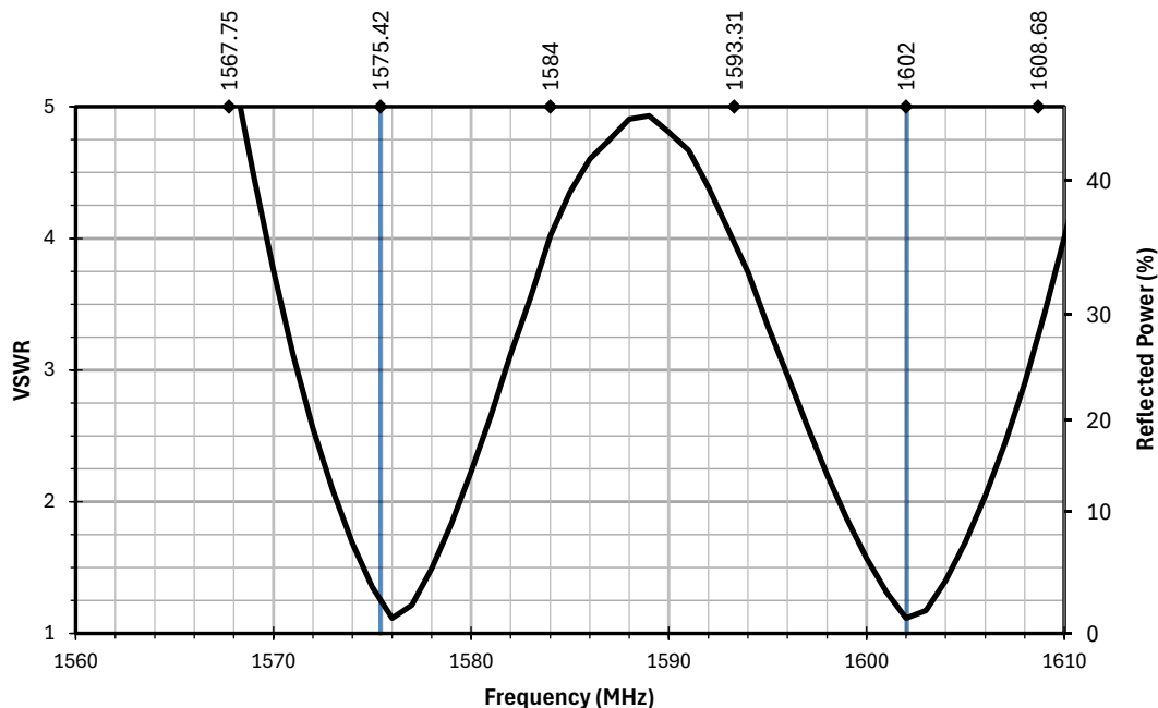
Figure 2. AC33182-1T Antenna VSWR with Frequency Band Highlights
