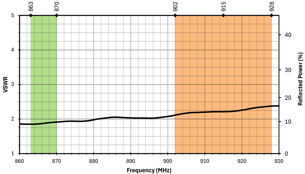
Figure 5. AC65001-NJ Antenna VSWR on Ground Plane
