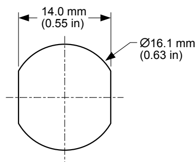
Figure 2. AC65001-NJ Antenna Mounting Dimensions
