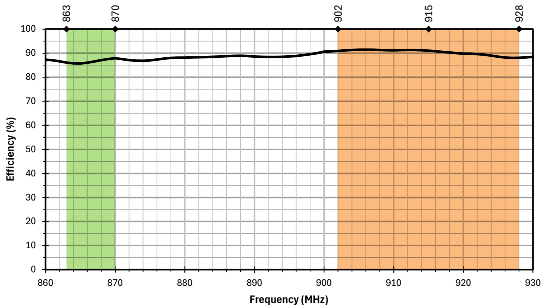
Figure 9. AC65001-NJ Antenna Efficiency on Ground Plane
