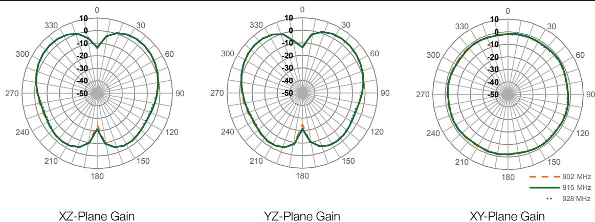
Figure 10. Radiation Patterns for AC65001-NJ Antenna on Ground Plane
