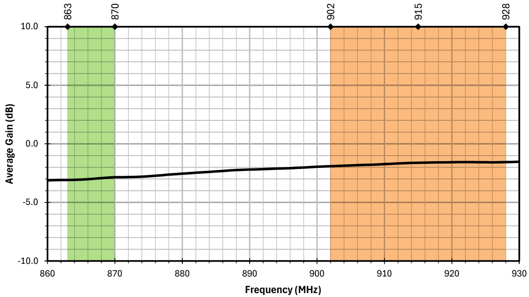
Figure 15. AC65001-NJ Antenna Average Gain, Free Space
