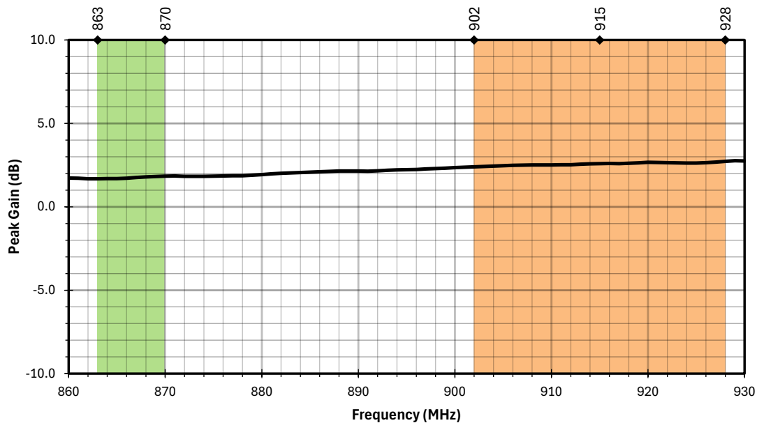
Figure 14. AC65001-NJ Antenna Peak Gain, Free Space
