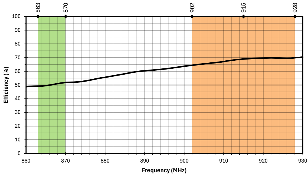
Figure 16. AC65001-NJ Antenna Efficiency, Free Space
