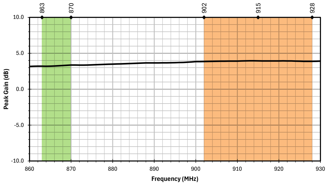
Figure 7. AC65001-NJ Antenna Peak Gain on Ground Plane
