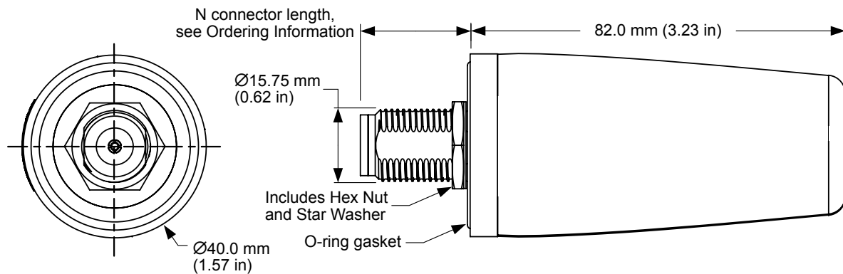
Figure 1. AC65001-NJ Antenna Dimensions
