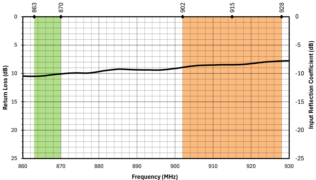
Figure 6. AC65001-NJ Antenna Return Loss on Ground Plane
