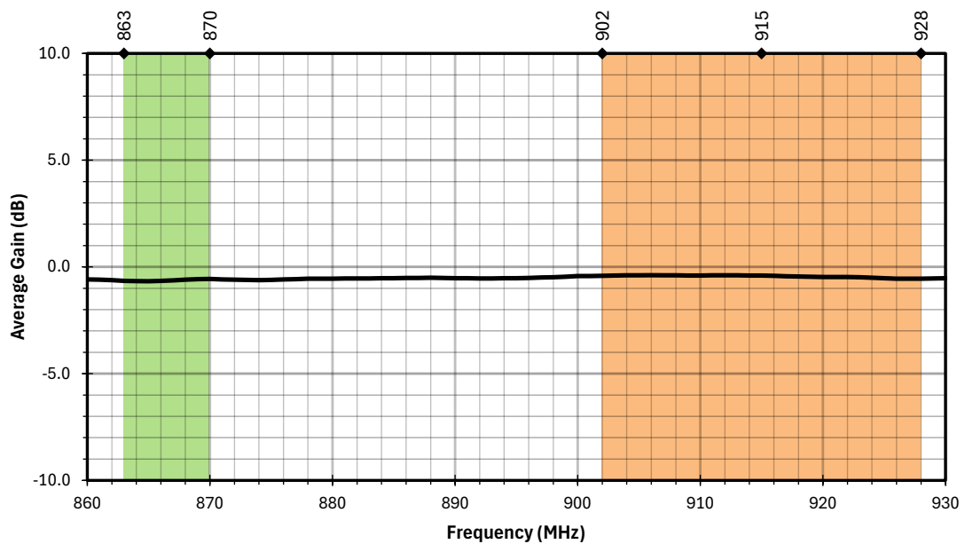
Figure 8. AC65001-NJ Antenna Average Gain on Ground Plane
