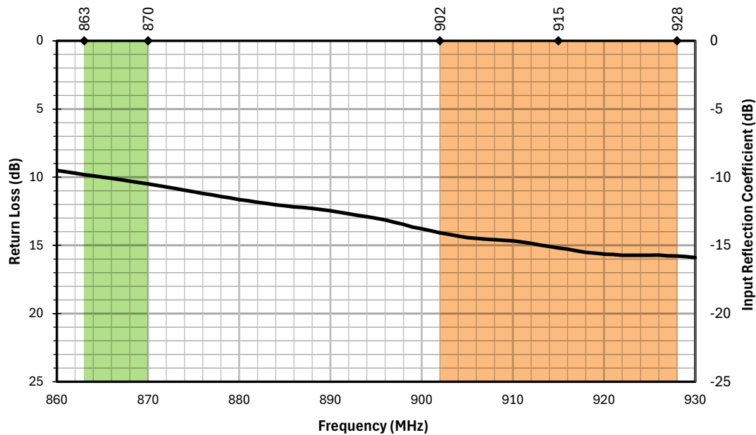
Figure 13. AC65001-NJ Antenna Return Loss, Free Space
