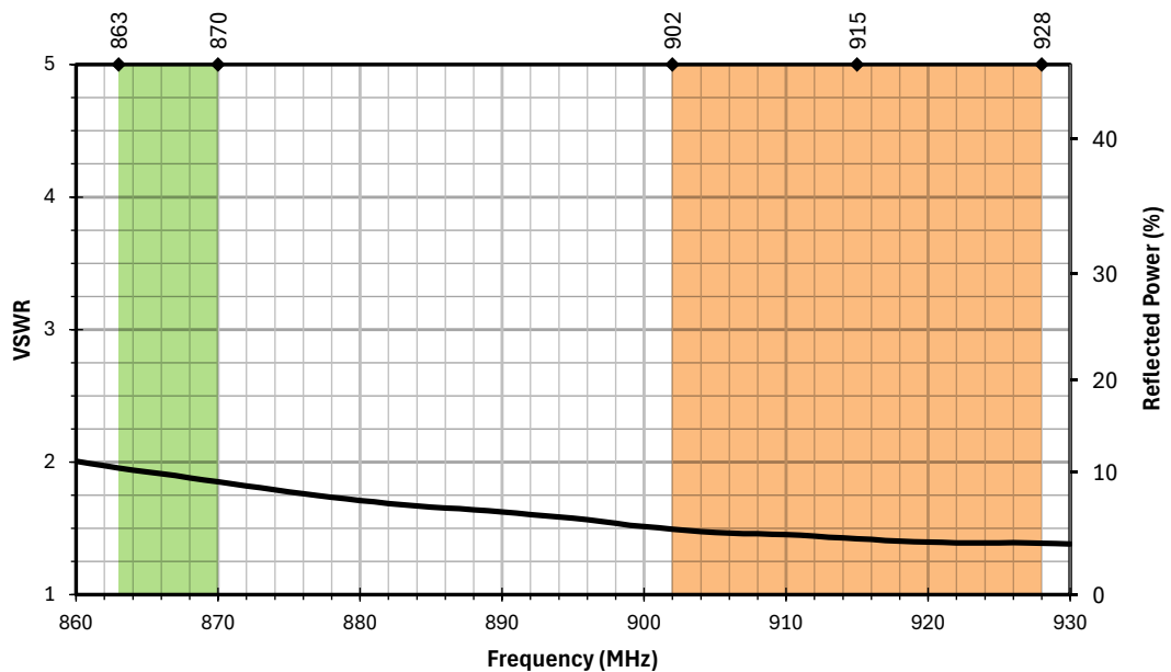
Figure 12. AC65001-NJ Antenna VSWR, Free Space
