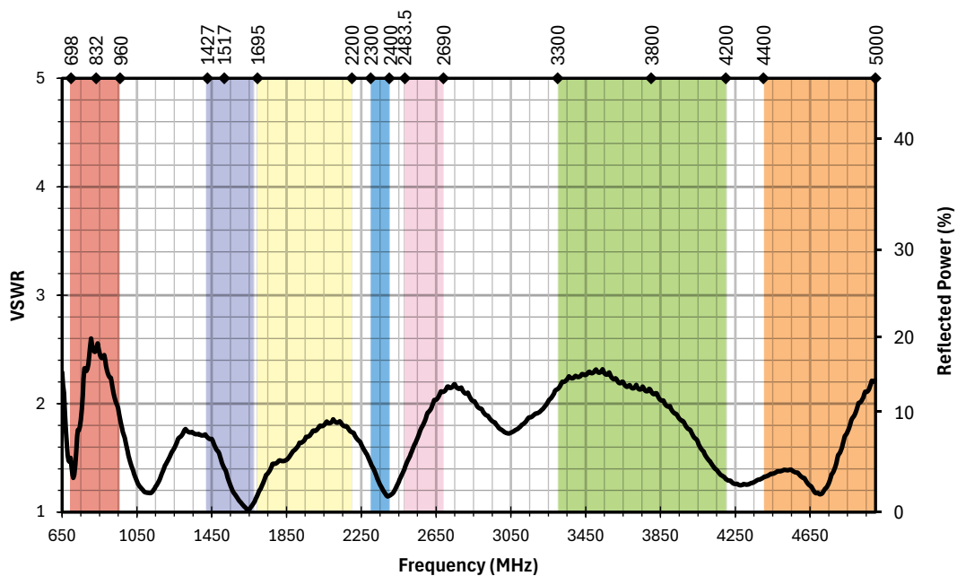
Figure 2. AC81001 Antenna VSWR
