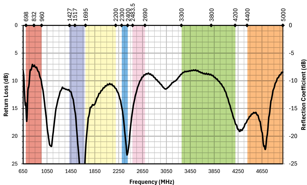
Figure 3. AC81001 Antenna Return Loss
