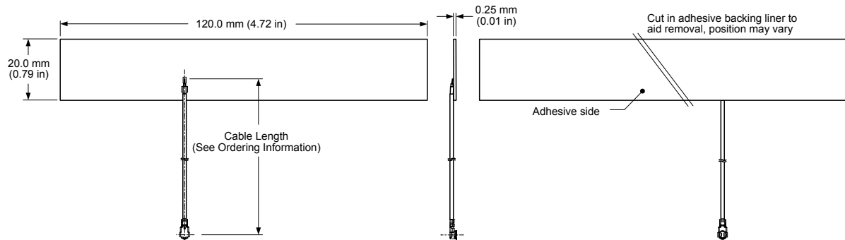
Figure 1. AC81001 Antenna Dimensions
