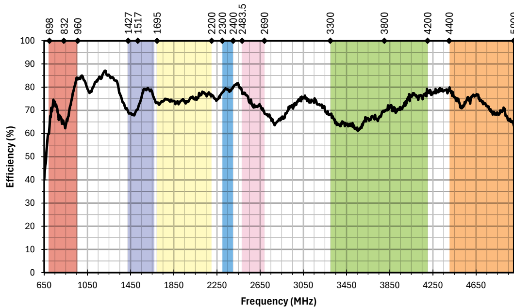
Figure 6. AC81001 Antenna Efficiency
