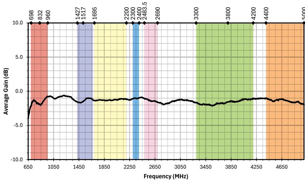
Figure 5. AC81001 Antenna Average Gain
