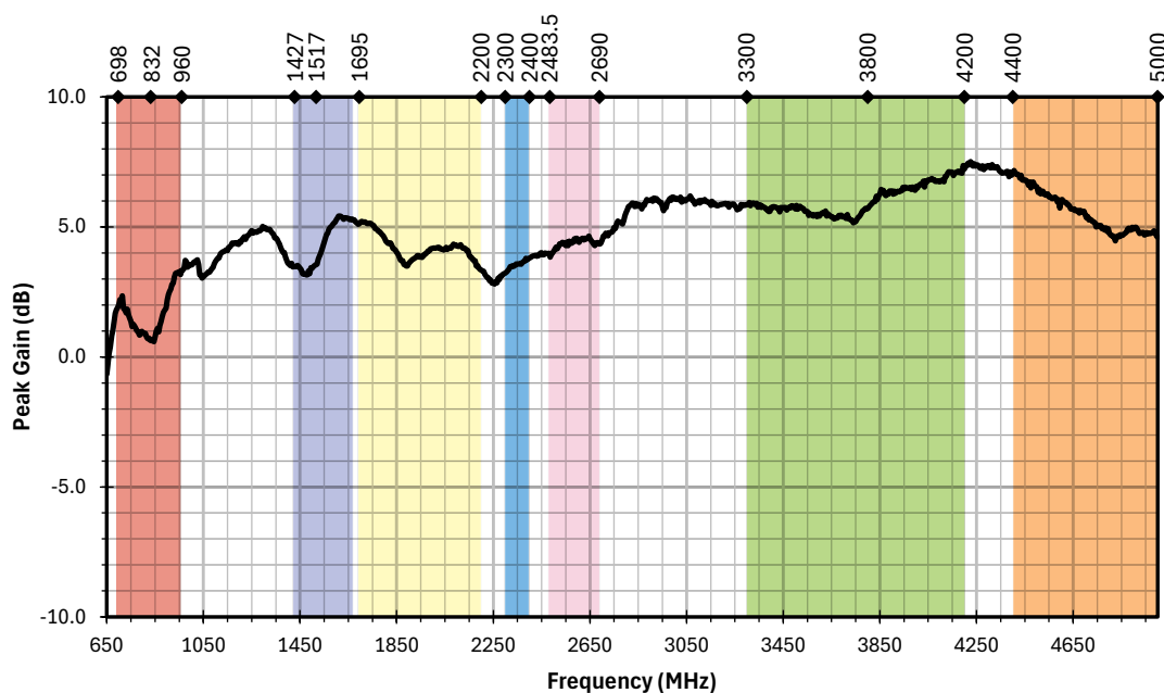
Figure 4. AC81001 Antenna Peak Gain
