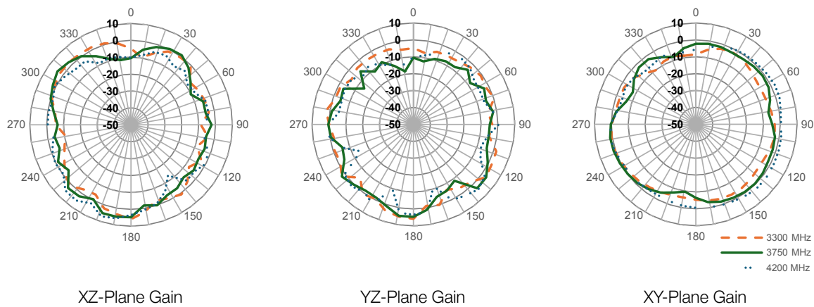
Figure 7. Radiation Patterns for the AC81001 Antenna
