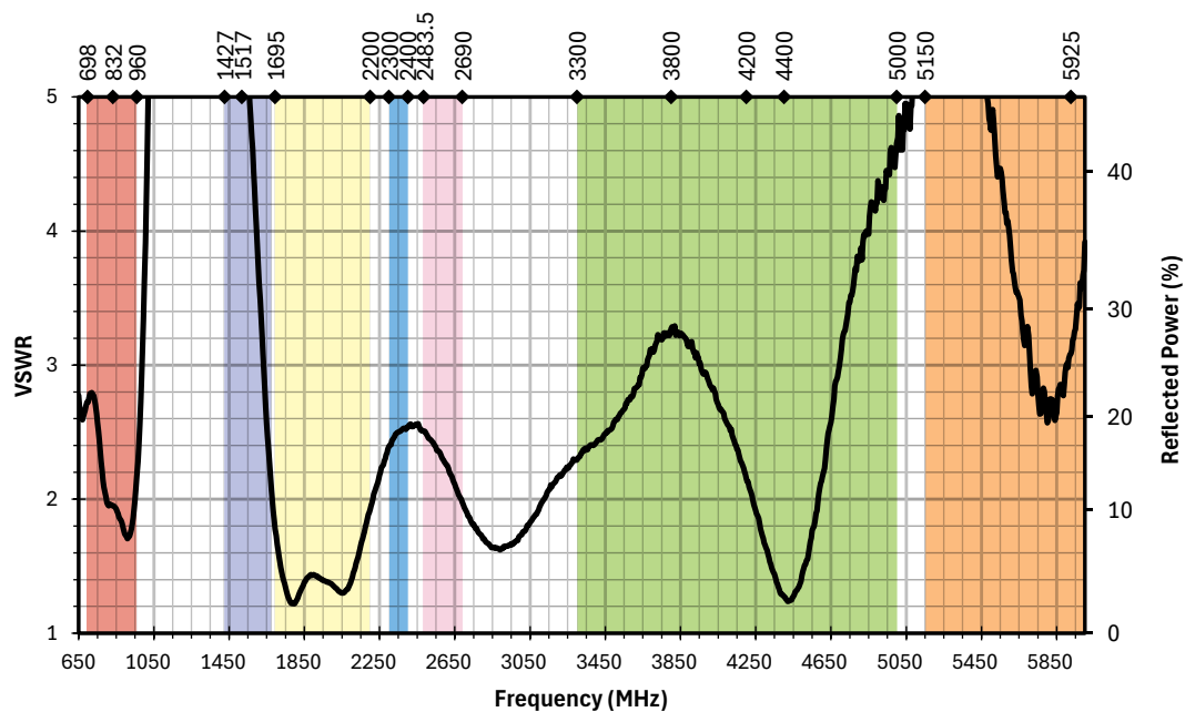
Figure 2. AC81003 Antenna VSWR
