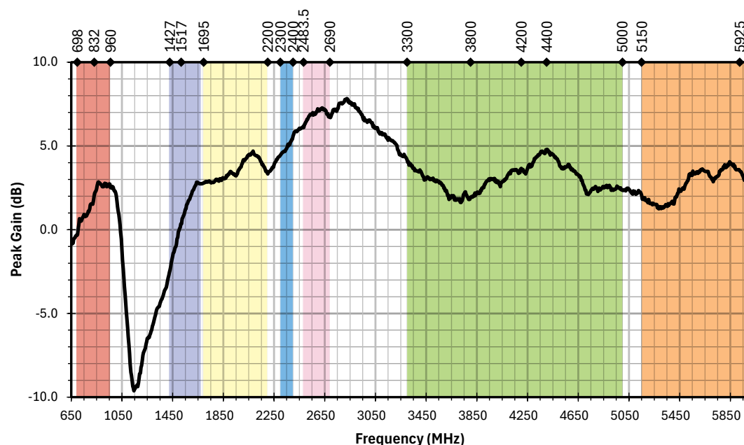
Figure 4. AC81003 Antenna Peak Gain
