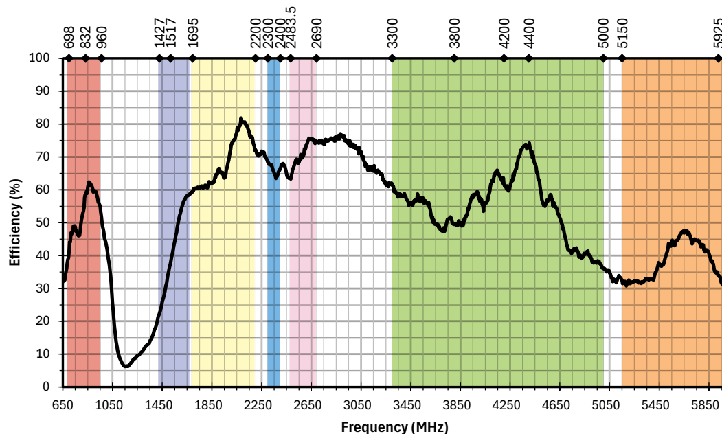
Figure 6. AC81003 Antenna Efficiency
