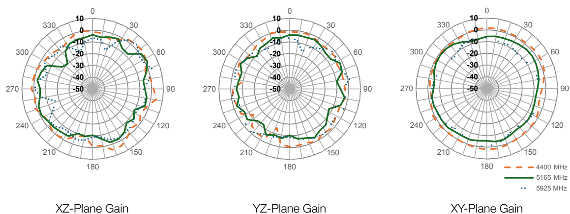
Figure 7. Radiation Patterns for the AC81003 Antenna
