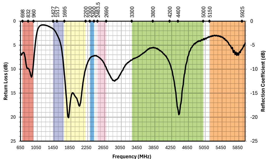
Figure 3. AC81003 Antenna Return Loss
