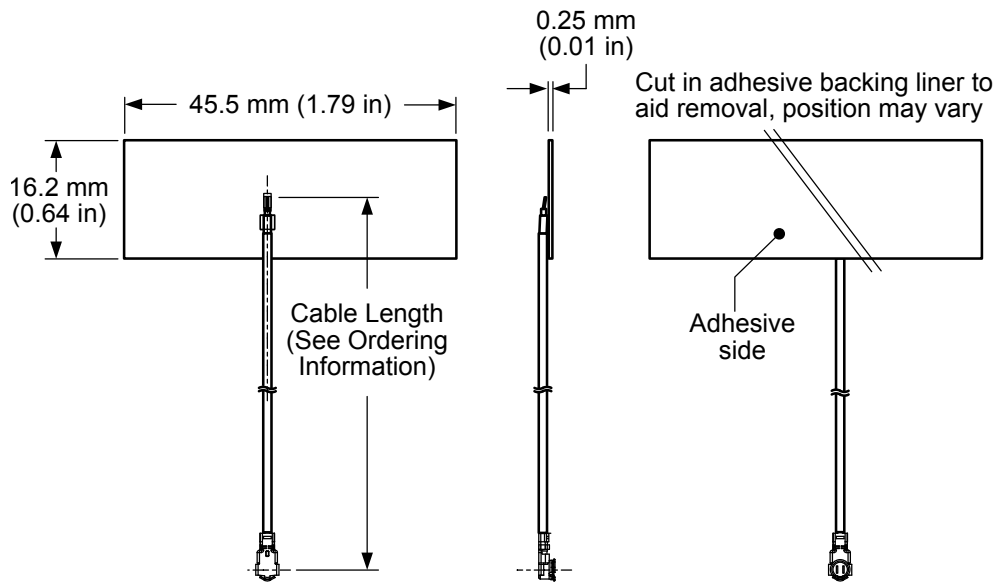
Figure 1. AC81003 Antenna Dimensions
