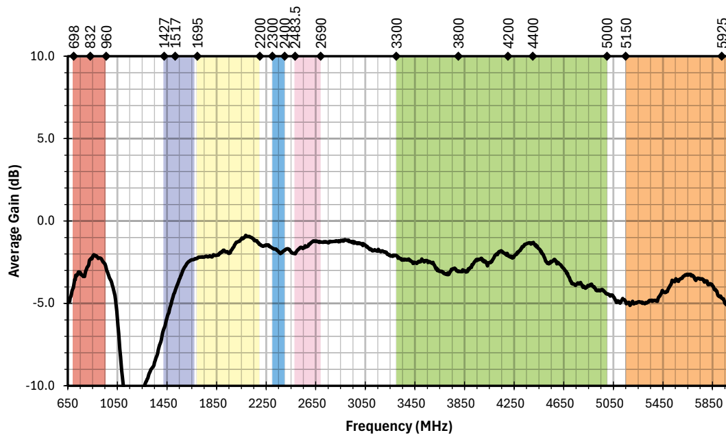
Figure 5. AC81003 Antenna Average Gain
