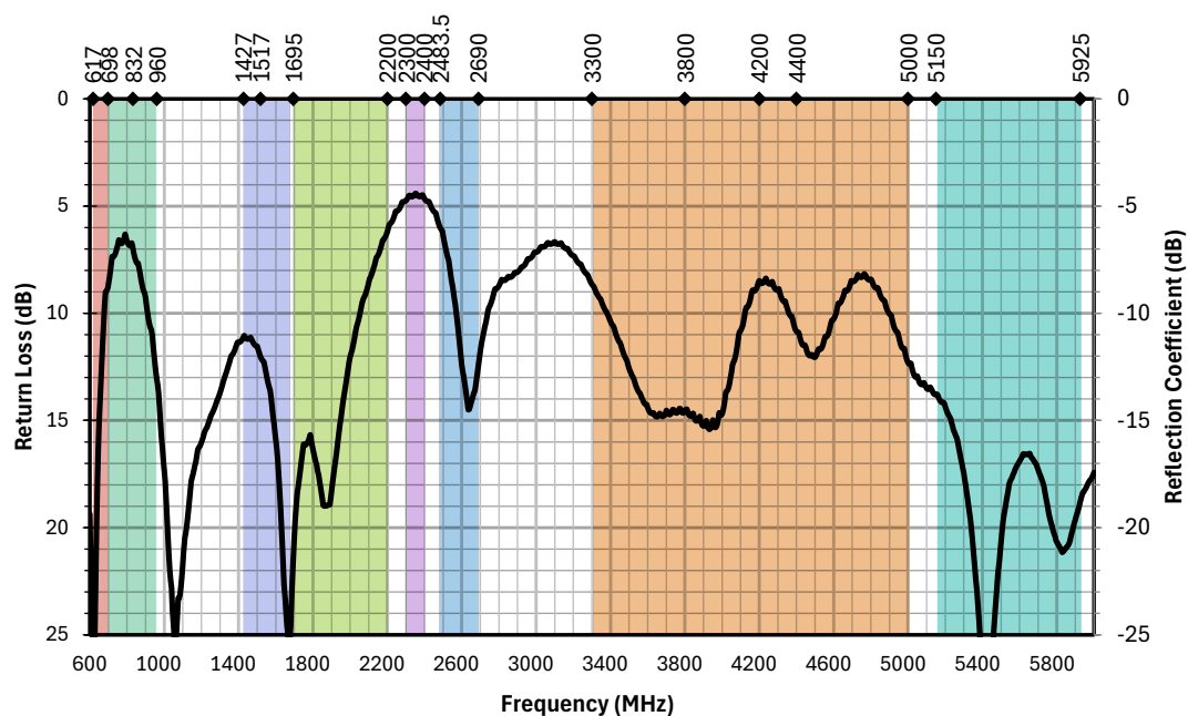
Figure 3. AC81005 Antenna Return Loss
