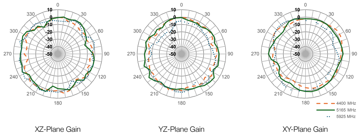
Figure 7. Radiation Patterns for the AC81005 Antenna
