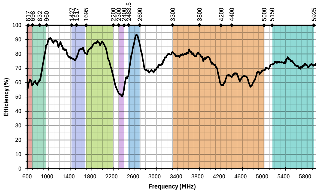
Figure 6. AC81005 Antenna Efficiency
