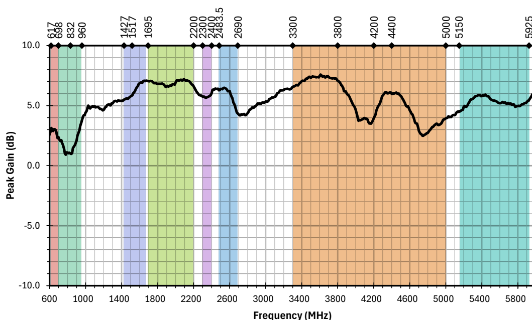
Figure 4. AC81005 Antenna Peak Gain
