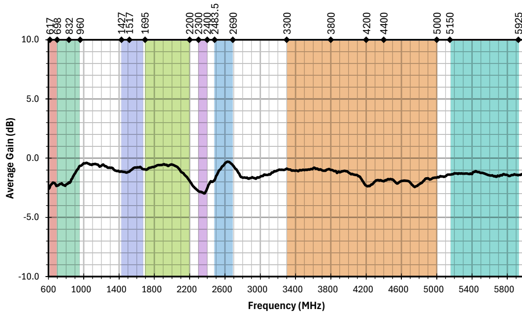
Figure 5. AC81005 Antenna Average Gain
