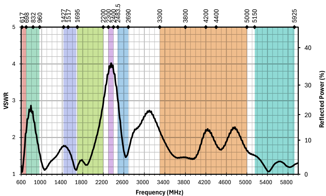
Figure 2. AC81005 Antenna VSWR
