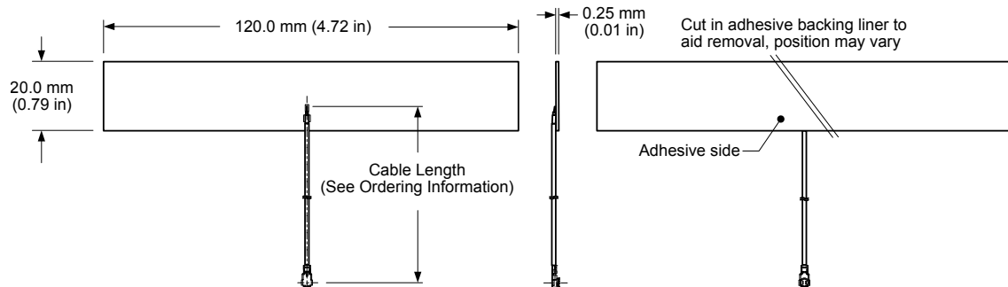
Figure 1. AC81005 Antenna Dimensions
