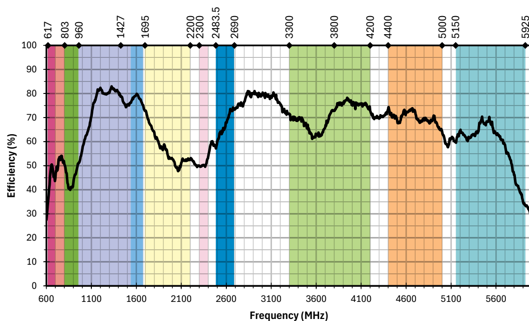
Figure 16. AC85003 Antenna Efficiency, Free Space
