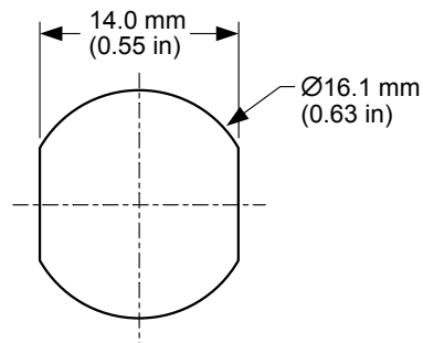
Figure 2. AC85003 Antenna Mounting Dimensions
