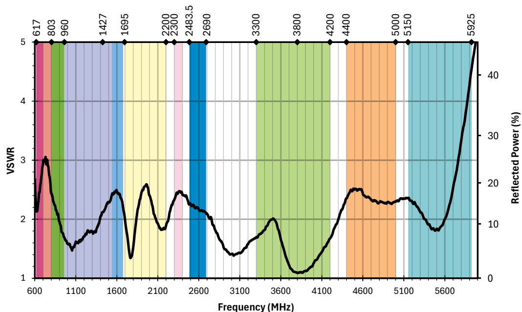
Figure 5. AC85003 Antenna VSWR on Ground Plane
