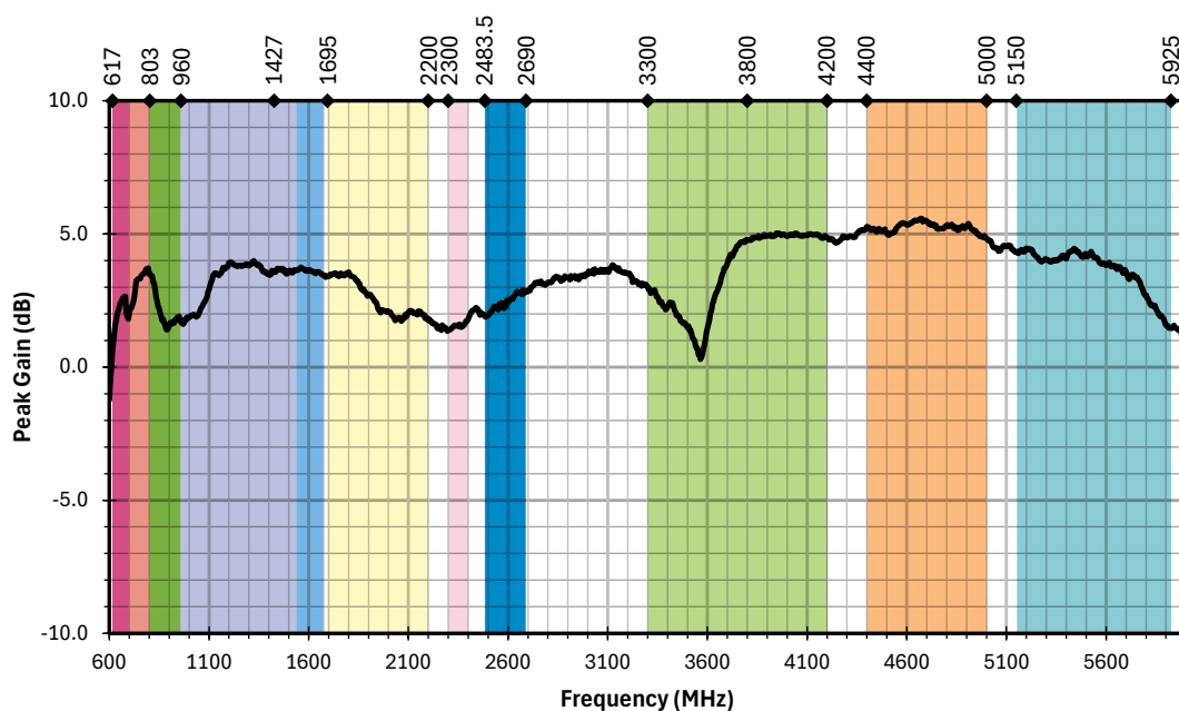
Figure 14. AC85003 Antenna Peak Gain, Free Space
