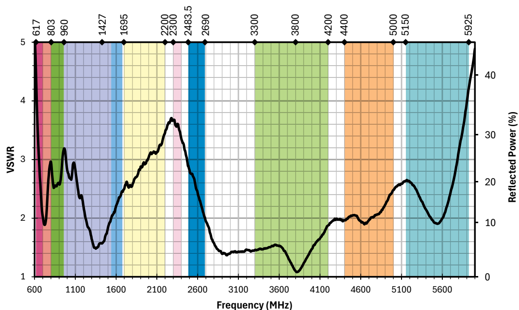
Figure 12. AC85003 Antenna VSWR, Free Space
