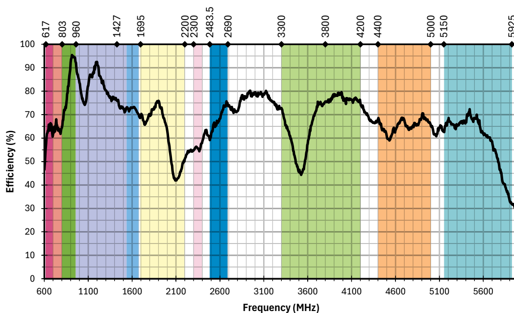
Figure 9. AC85003 Antenna Efficiency on Ground Plane
