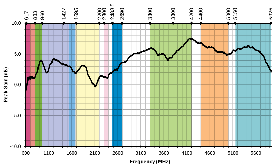
Figure 7. AC85003 Antenna Peak Gain on Ground Plane
