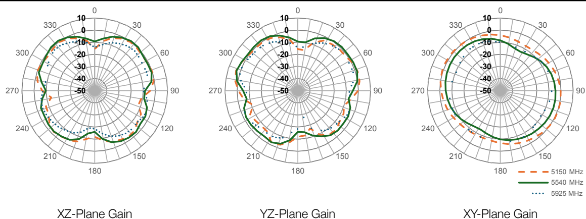
Figure 10. Radiation Patterns for AC85003 Antenna on Ground Plane
