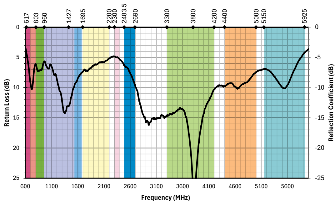
Figure 13. AC85003 Antenna Return Loss, Free Space
