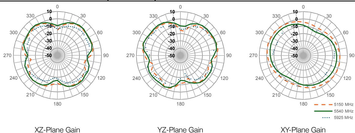
Figure 17. Radiation Patterns for AC85003 Antenna in Free Space
