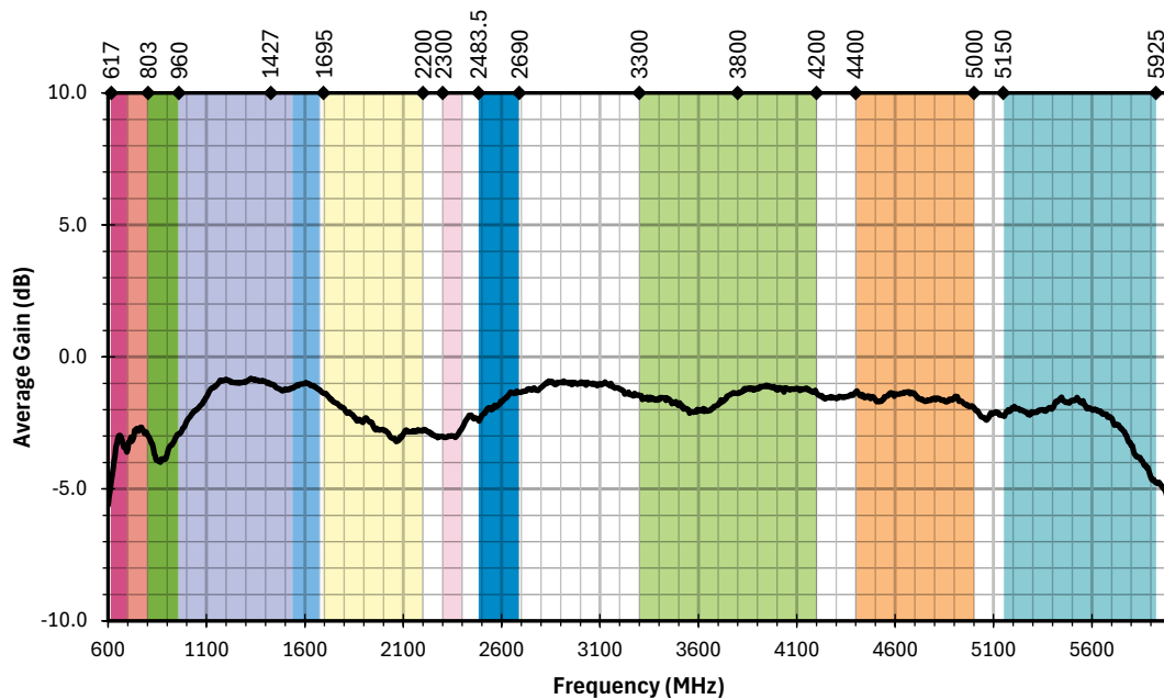
Figure 15. AC85003 Antenna Average Gain, Free Space
