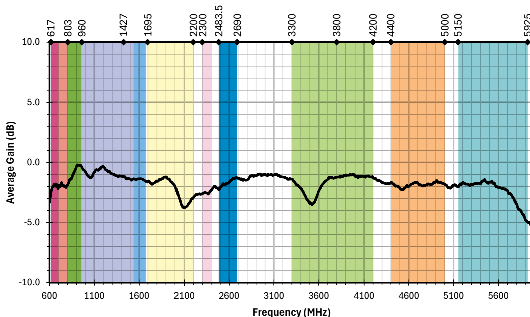
Figure 8. AC85003 Antenna Average Gain on Ground Plane
