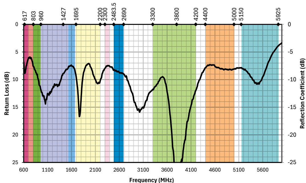
Figure 6. AC85003 Antenna Return Loss on Ground Plane
