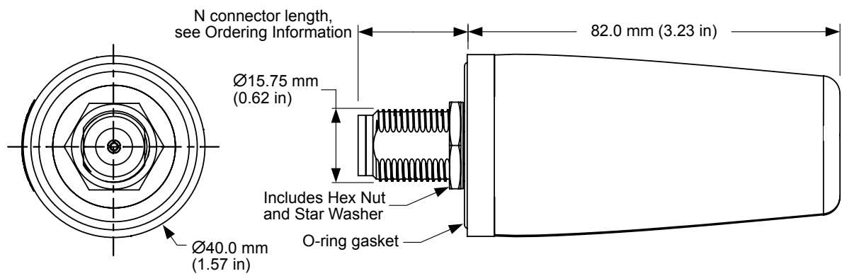
Figure 1. AC85003 Antenna Dimensions
