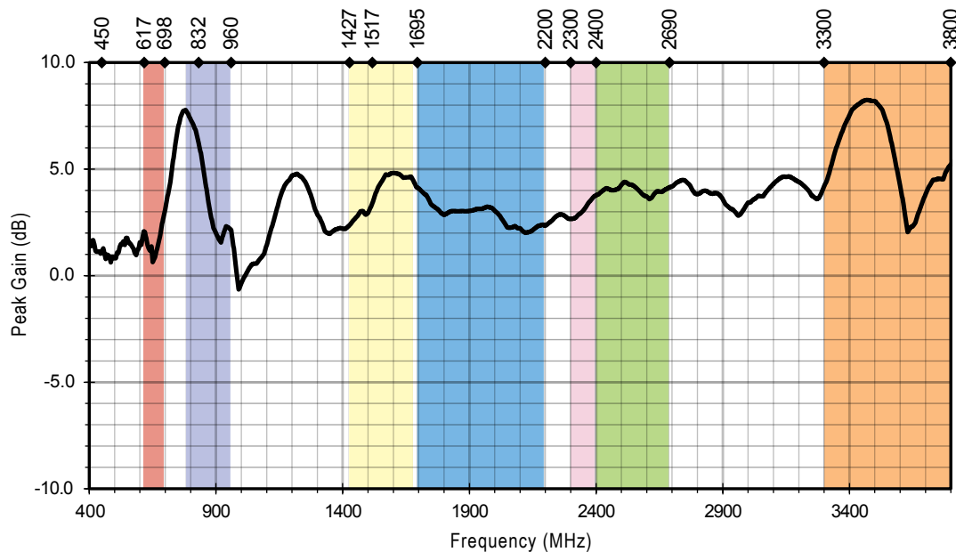
Figure 6. AC94541 Antenna Peak Gain on Ground Plane
