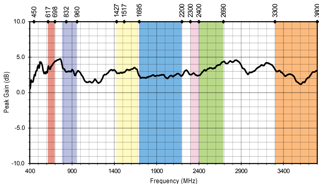
Figure 13. AC94541 Antenna Peak Gain, Free Space
