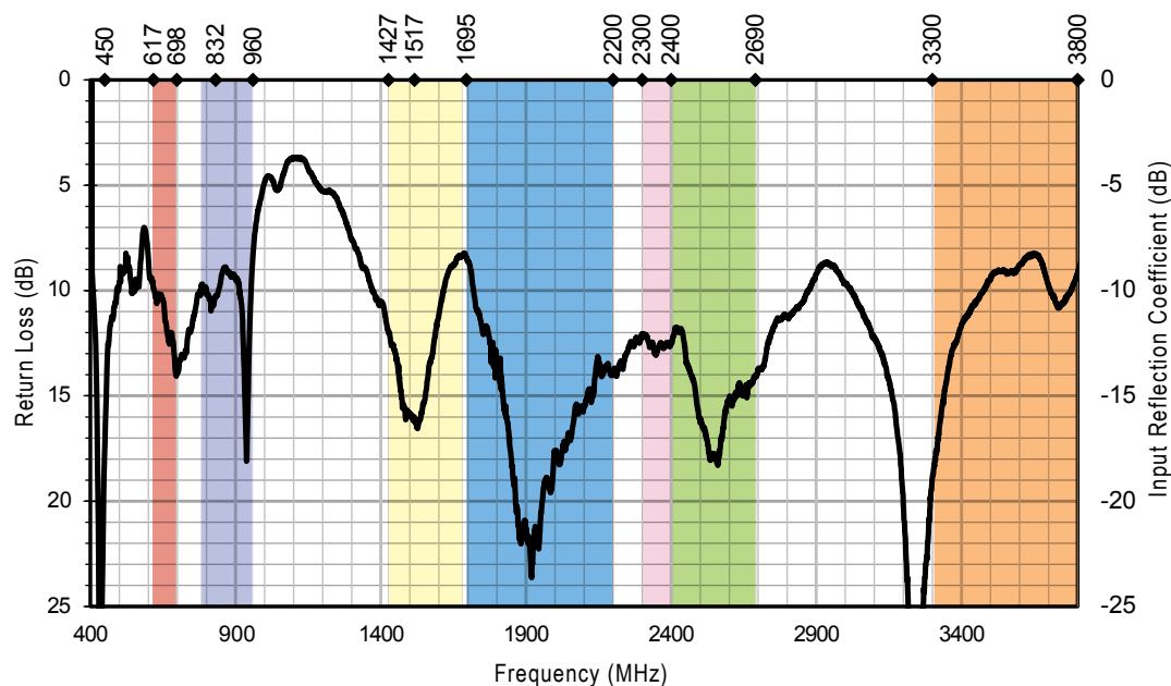
Figure 12. AC94541 Antenna Return Loss, Free Space
