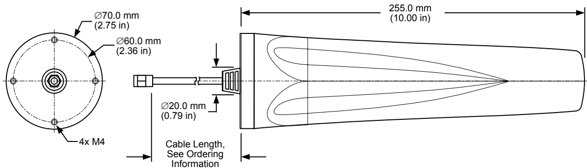
Figure 1. AC94541 Antenna Dimensions
