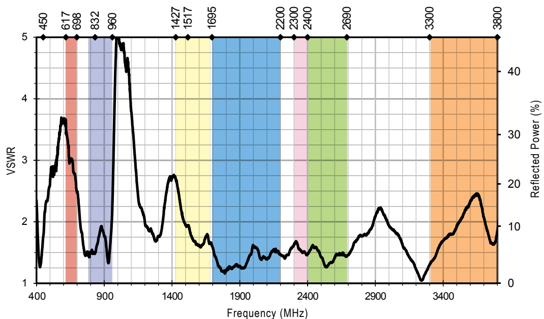
Figure 4. AC94541 Antenna VSWR on Ground Plane
