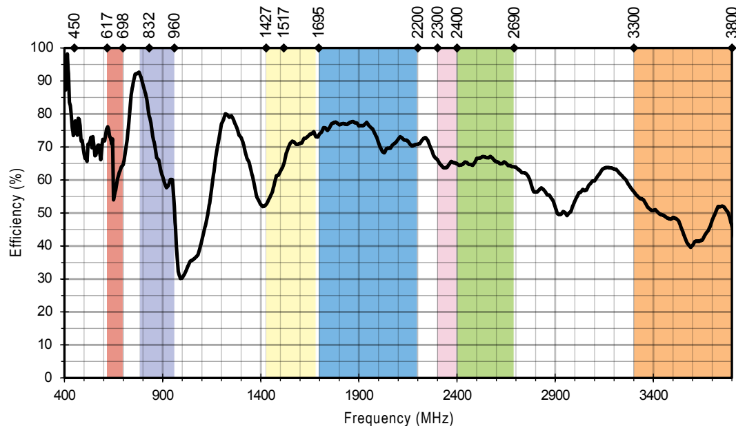
Figure 8. AC94541 Antenna Radiation Efficiency on Ground Plane
