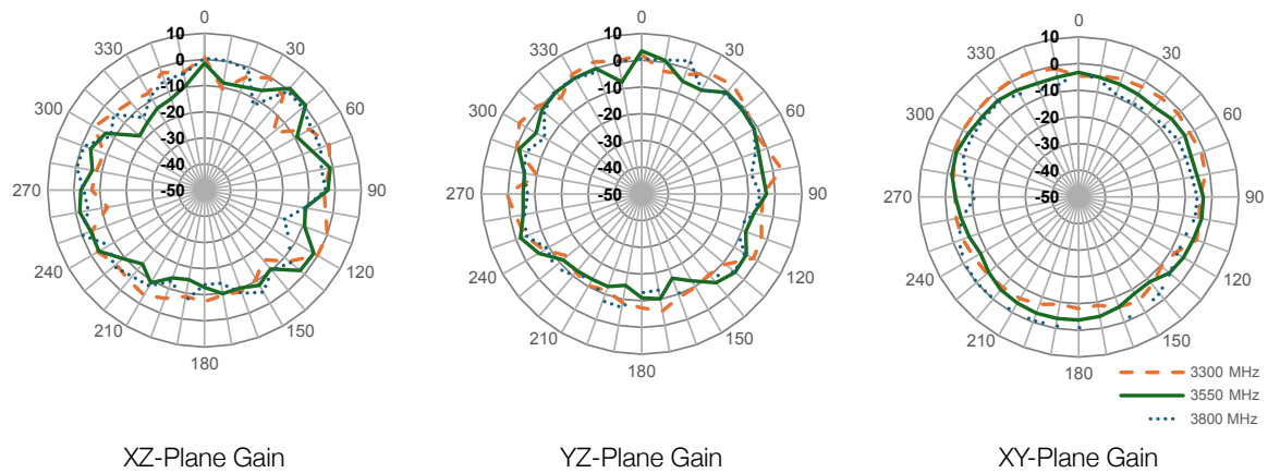
Figure 9. Radiation Patterns for AC94541 Antenna on Ground Plane
