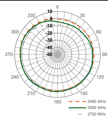
XY-Plane Gain
