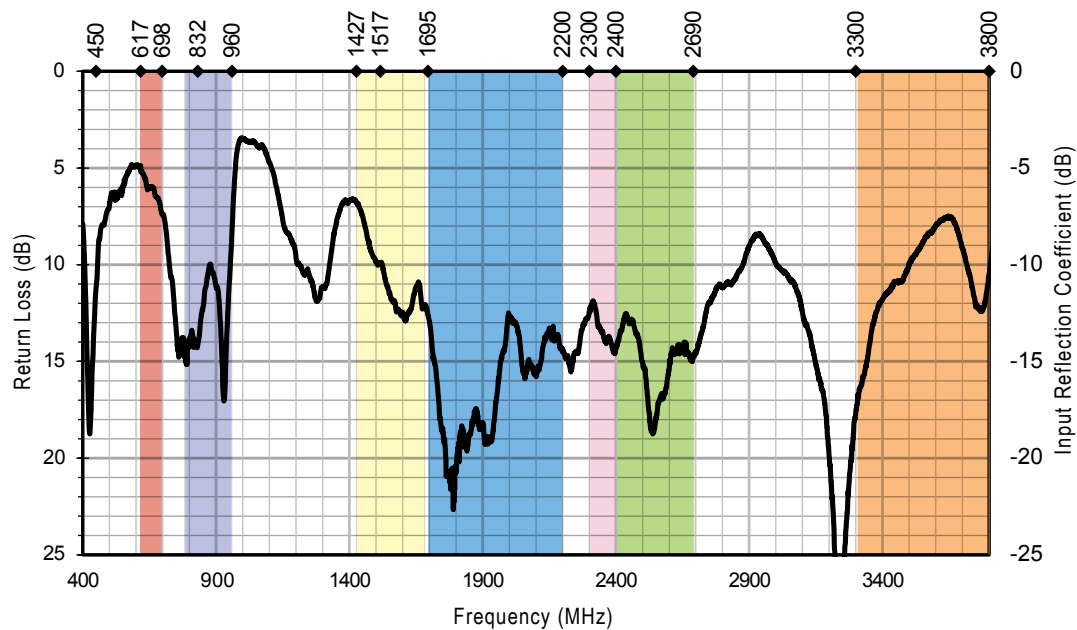
Figure 5. AC94541 Antenna Return Loss on Ground Plane
