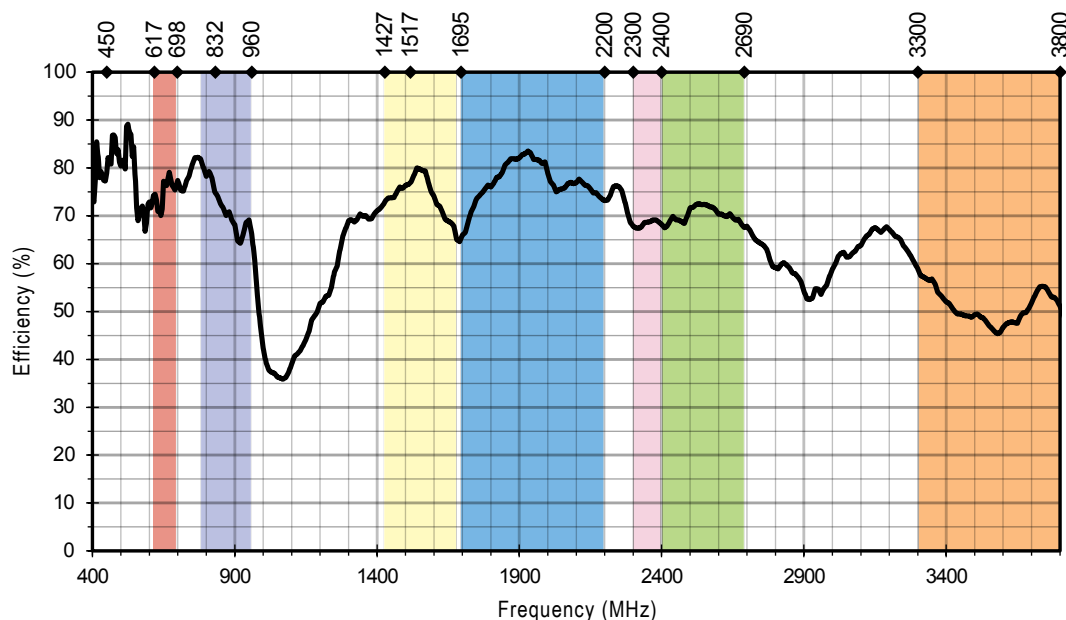
Figure 15. AC94541 Antenna Radiation Efficiency, Free Space
