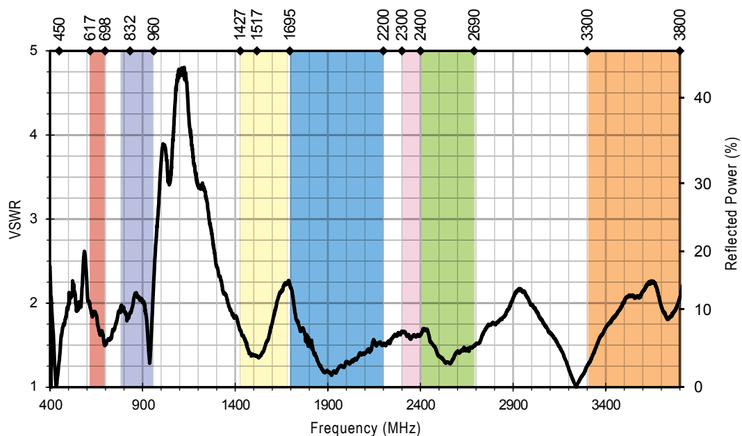
Figure 11. AC94541 Antenna VSWR, Free Space
