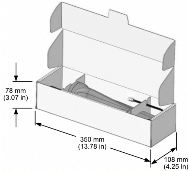
Figure 19. AC94541 Antenna Packaging Dimensions
