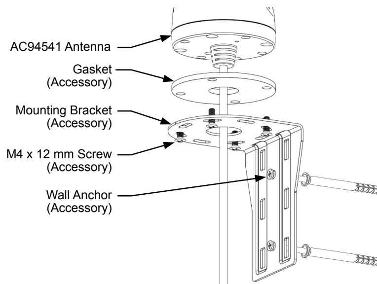
Figure 18. AC94541 Antenna Mounting Methods
