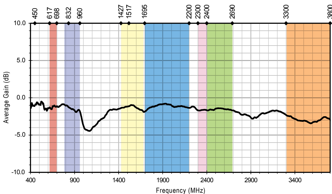
Figure 14. AC94541 Antenna Average Gain, Free Space
