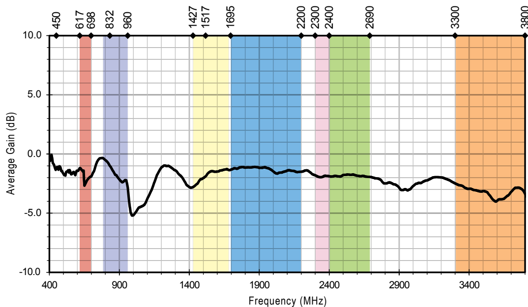
Figure 7. AC94541 Antenna Average Gain on Ground Plane
