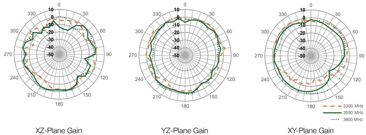
Figure 16. Radiation Patterns for AC94541 Antenna in Free Space
